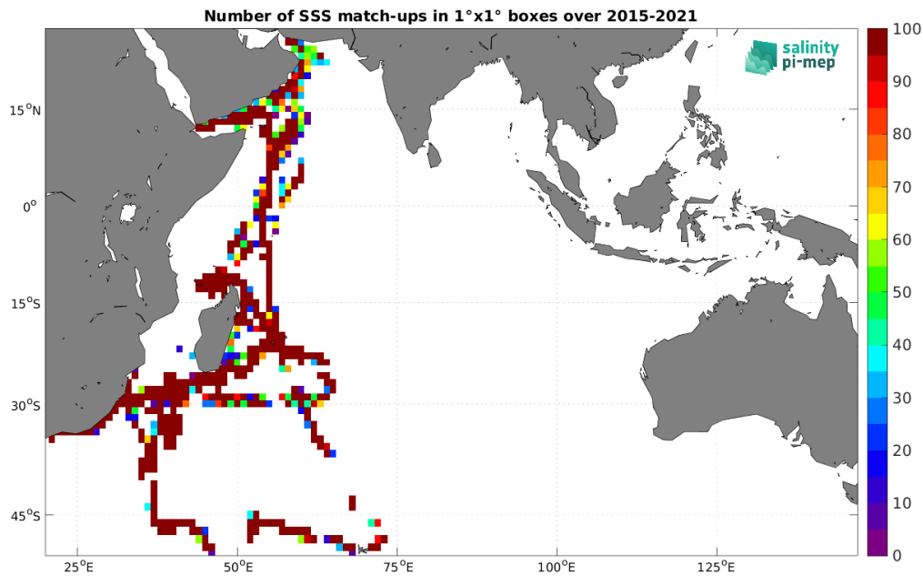
Figure 4: Number of SSS match-ups between TSG (GOSUD-Research-vessel) SSS and the SMAP SSS L2 v5.0 (JPL) SSS product for the Indian Ocean Pi-MEP region over 1^{\circ} \times 1^{\circ} boxes and for the full satellite product period.
