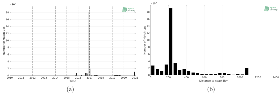
Figure 1: Number of match-ups between TSG (GOSUD-Research-vessel) and SMAP SSS L2 v5.0 (JPL) SSS as a function of time (a) and as function of the distance to coast (b) over the Indian Ocean Pi-MEP region and for the full satellite product period.
