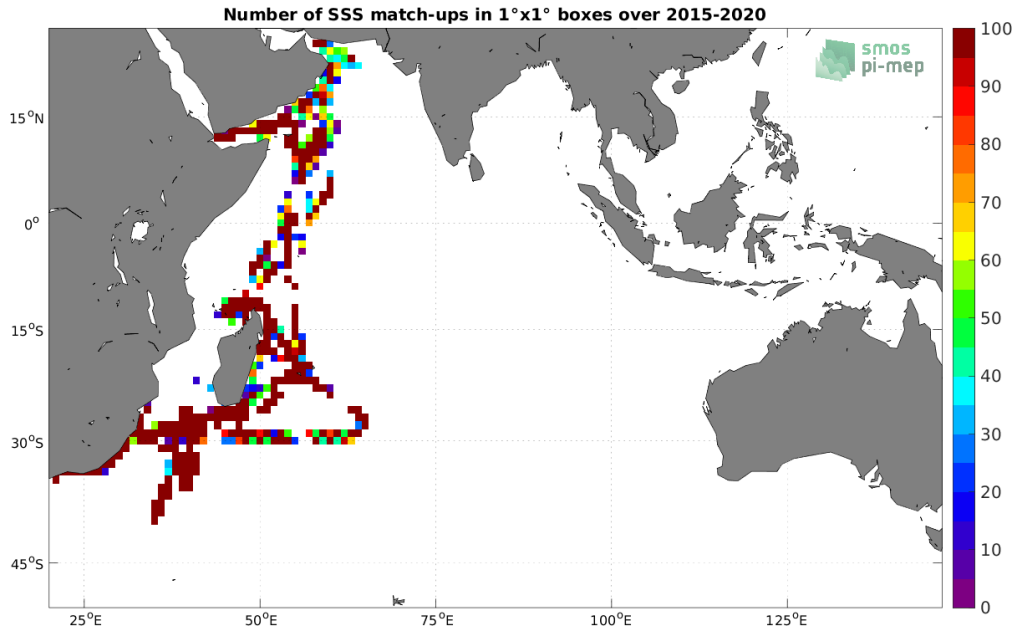
Figure 4: Number of SSS match-ups between TSG (GOSUD-Research-vessel) SSS and the SMAP SSS L2 v5.0 (JPL) SSS product for the Indian Ocean Pi-MEP region over 1^\circ \times 1^\circ boxes and for the full satellite product period.
