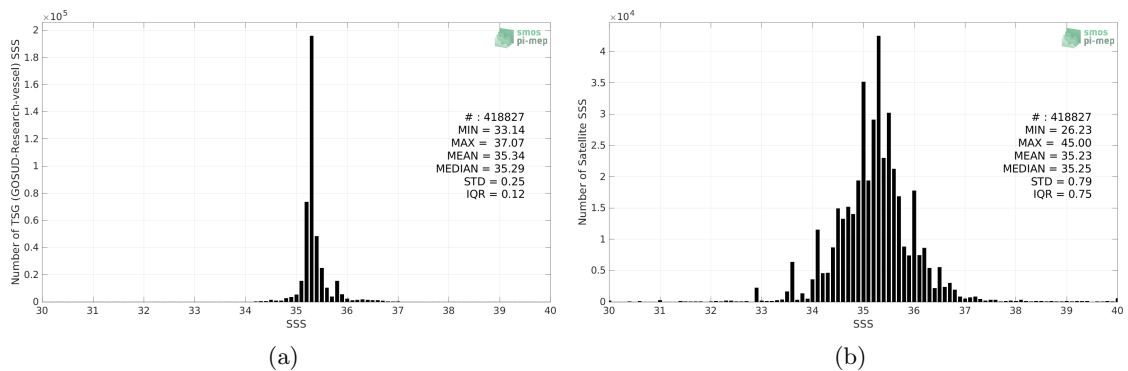
Figure 2: Histograms of SSS from TSG (GOSUD-Research-vessel) (a) and SMAP SSS L2 v5.0 (JPL) (b) considering all match-up pairs per bins of 0.1 over the Indian Ocean Pi-MEP region and for the full satellite product period.
