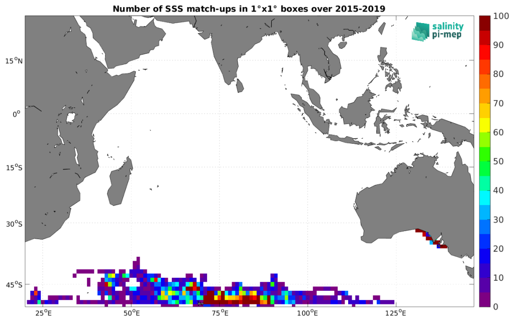
Figure 4: Number of SSS match-ups between Marine mammals SSS and the SMAP SSS L2 v5.0 (JPL) SSS product for the Indian Ocean Pi-MEP region over 1^\circ \times 1^\circ boxes and for the full satellite product period.
