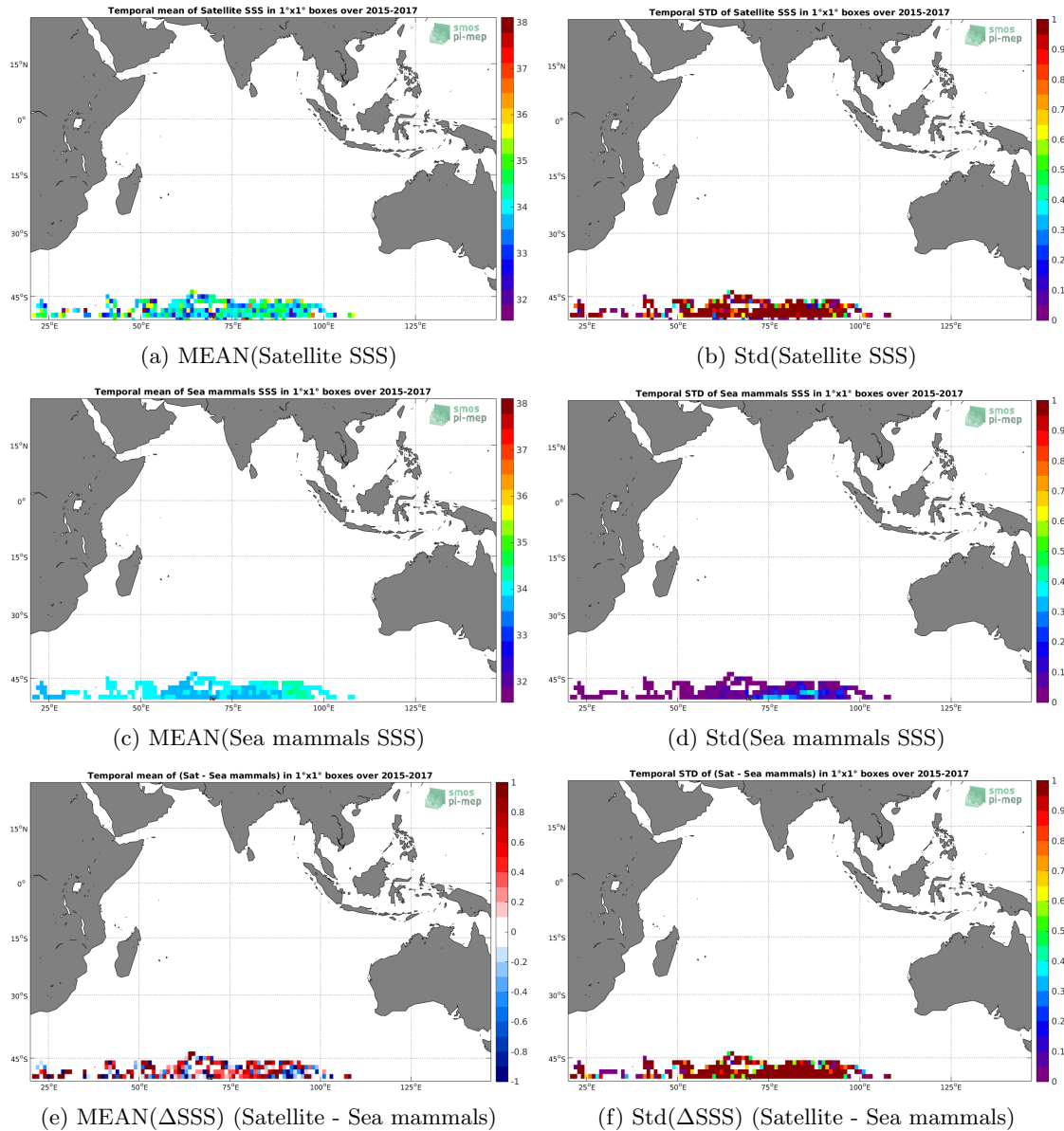
Figure 6: Temporal mean (left) and Std (right) of SSS from SMAP SSS L2 v5.0 (JPL) (top), Sea mammals (middle), and of \Delta SSS (Satellite - Sea mammals). Only match-up pairs are used to generate these maps.
