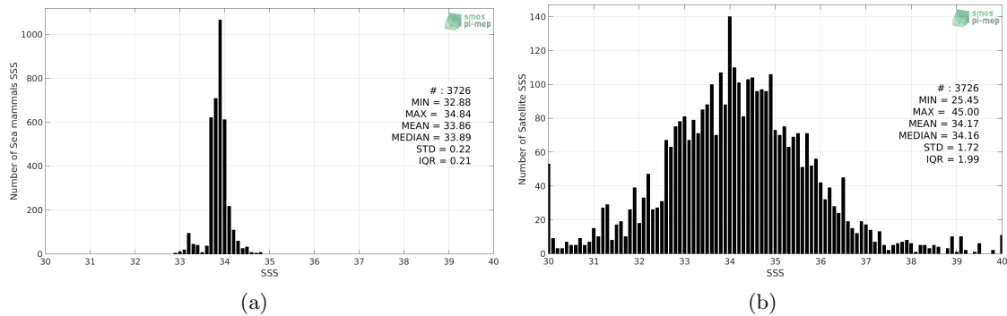
Figure 2: Histograms of SSS from Sea mammals (a) and SMAP SSS L2 v5.0 (JPL) (b) considering all match-up pairs per bins of 0.1 over the Indian Ocean Pi-MEP region and for the full satellite product period.
