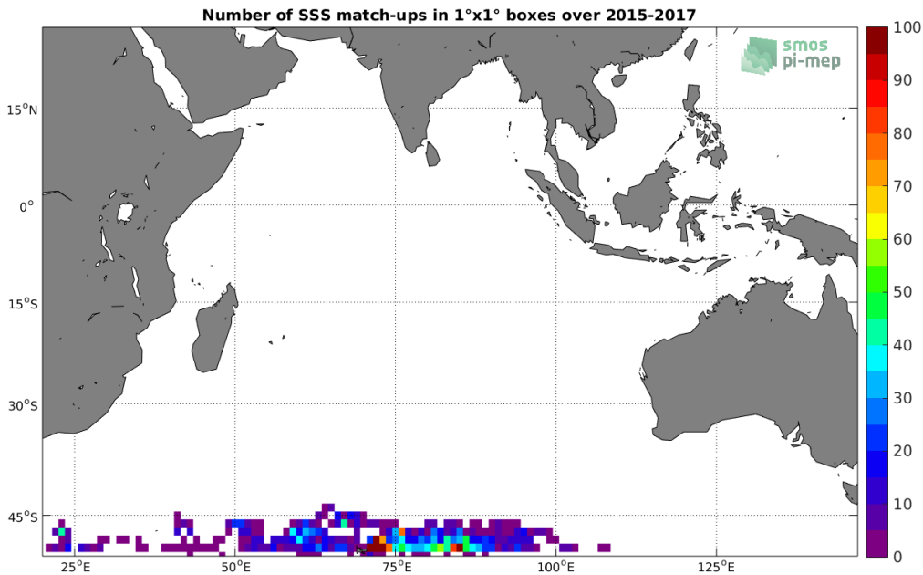
Figure 4: Number of SSS match-ups between Sea mammals SSS and the SMAP SSS L2 v5.0 (JPL) SSS product for the Indian Ocean Pi-MEP region over 1°x1° boxes and for the full satellite product period.
