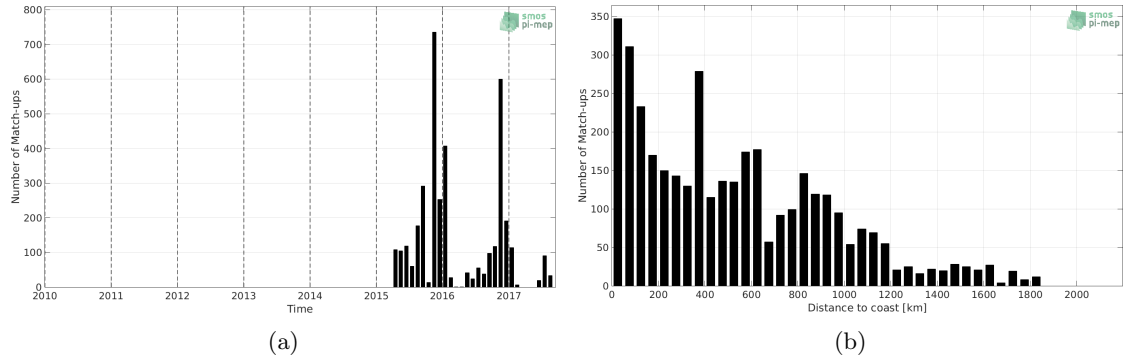
Figure 1: Number of match-ups between Sea mammals and SMAP SSS L2 v5.0 (JPL) SSS as a function of time (a) and as function of the distance to coast (b) over the Indian Ocean Pi-MEP region and for the full satellite product period.
