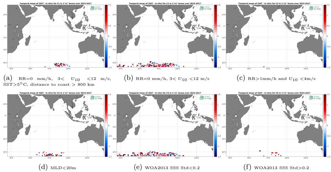
Figure 12: Temporal mean gridded over spatial boxes of size 1^{\circ}\times 1^{\circ} of \Delta\text{SSS} (SMAP SSS L2 v5.0 (JPL) - Sea mammals) for 6 different subdatasets corresponding to:RR=0 mm/h, 3 < U_{10} < 12 m/s, SST > 5^{\circ}\text{C} , distance to coast > 800 km (a), RR=0 mm/h, 3 < U_{10} < 12 m/s (b), RR > 1\text{mm/h} and U_{10} < 4\text{m/s} (c),MLD < 20\text{m} (d),WOA2013 SSS Std < 0.2 (e),WOA2013 SSS Std > 0.2 (f).
