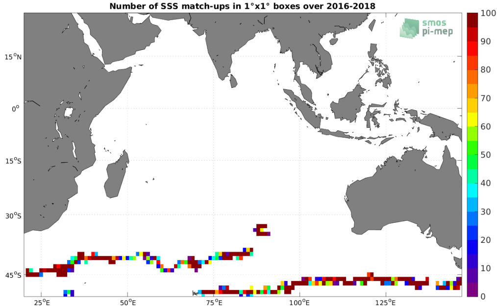
Figure 3: Number of SSS match-ups between Surface drifters SSS and the SMAP SSS L2 v5.0 (JPL) SSS product for the Indian Ocean Pi-MEP region over 1^\circ \times 1^\circ boxes and for the full satellite product period.
