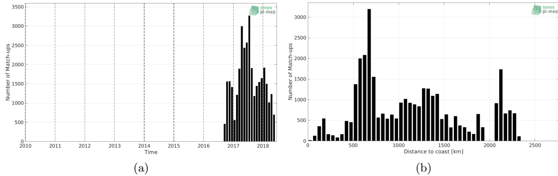
Figure 1: Number of match-ups between Surface drifters and SMAP SSS L2 v5.0 (JPL) SSS as a function of time (a) and as function of the distance to coast (b) over the Indian Ocean Pi-MEP region and for the full satellite product period.
