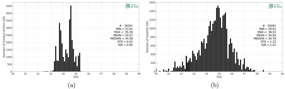
Figure 2: Histograms of SSS from Surface drifters (a) and SMAP SSS L2 v5.0 (JPL) (b) considering all match-up pairs per bins of 0.1 over the Indian Ocean Pi-MEP region and for the full satellite product period.
