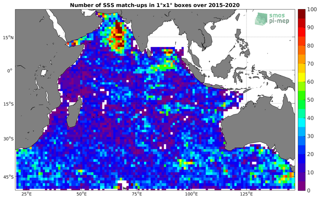
Figure 4: Number of SSS match-ups between Argo SSS and the SMAP SSS L2 v5.0 (JPL) SSS product for the Indian Ocean Pi-MEP region over 1°x1° boxes and for the full satellite product period.
