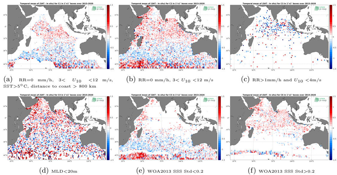
Figure 12: Temporal mean gridded over spatial boxes of size 1^\circ \times 1^\circ of \Delta SSS (SMAP SSS L2 v5.0 (JPL) - Argo) for 6 different subdatasets corresponding to: RR=0 mm/h, 3 < U_{10} < 12 m/s, SST > 5°C, distance to coast > 800 km (a), RR=0 mm/h, 3 < U_{10} < 12 m/s (b), RR > 1mm/h and U_{10} < 4 m/s (c), MLD < 20m (d), WOA2013 SSS Std < 0.2 (e), WOA2013 SSS Std > 0.2 (f).
