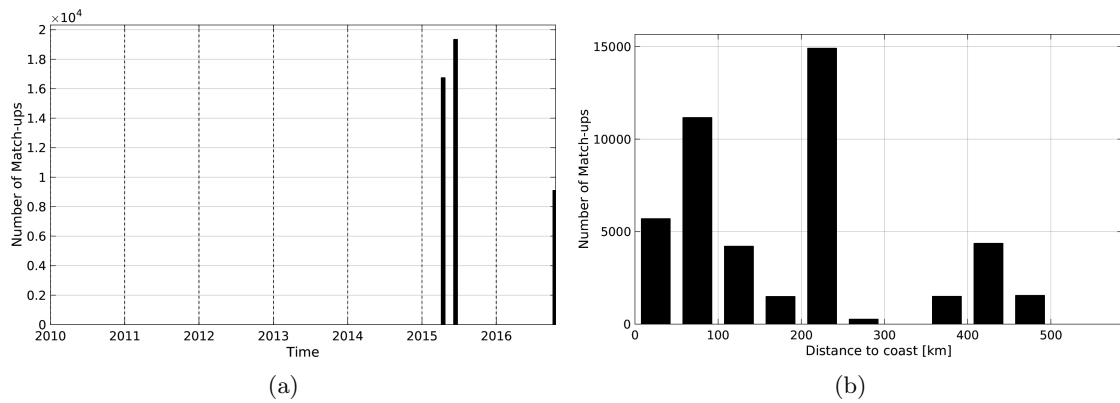
Figure 1: Number of match-ups between TSG-SAMOS and SMAP-L2-JPL-V4 SSS as a function of time (a) and as function of the distance to coast (b) over the Indian Ocean Pi-MEP region and for the full satellite product period.
