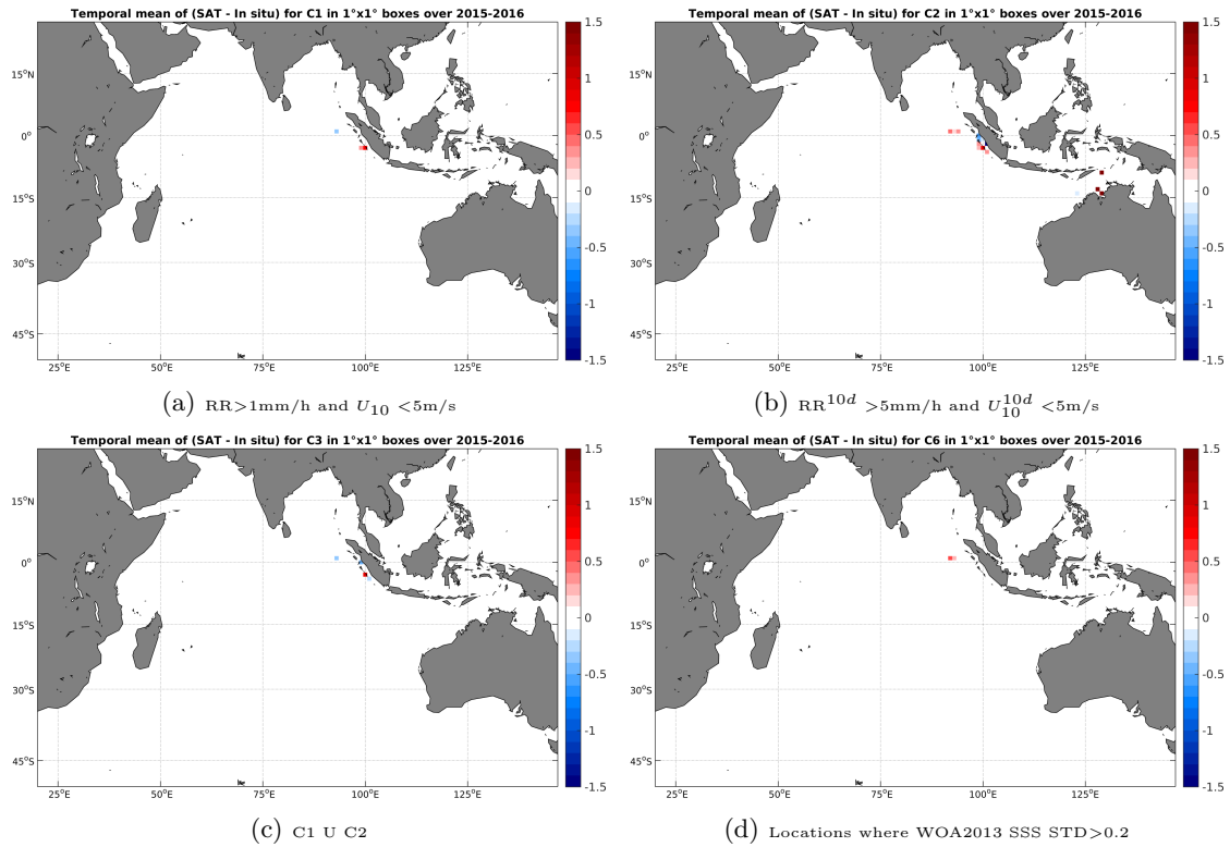
Figure 12: Temporal mean gridded over spatial boxes of size 1^\circ \times 1^\circ of \Delta SSS (SMAP-L2-JPL-V4 - TSG-SAMOS) for 4 different subdatasets corresponding to:RR > 1mm/h and U_{10} < 5 m/s (a), RR^{10d} > 5 mm/h and U_{10}^{10d} < 5 m/s (b), C1 U C2 (c),Locations where WOA2013 SSS STD > 0.2 (d).
