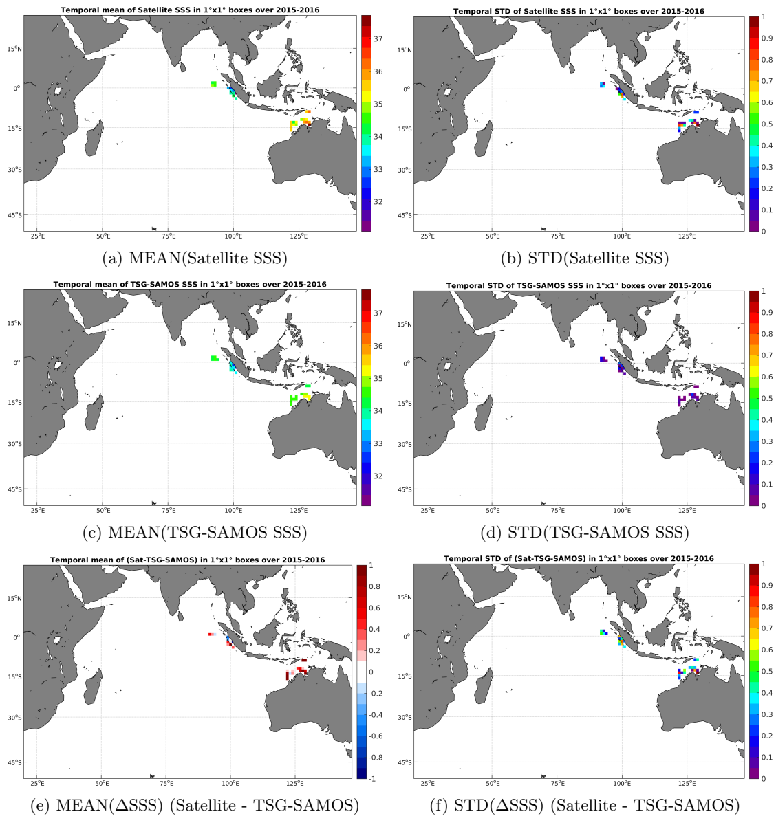
Figure 6: Temporal mean (left) and STD (right) of SSS from SMAP-L2-JPL-V4 (top), TSG-SAMOS (middle), and of \Delta SSS (Satellite - TSG-SAMOS). Only match-up pairs are used to generate these maps.
