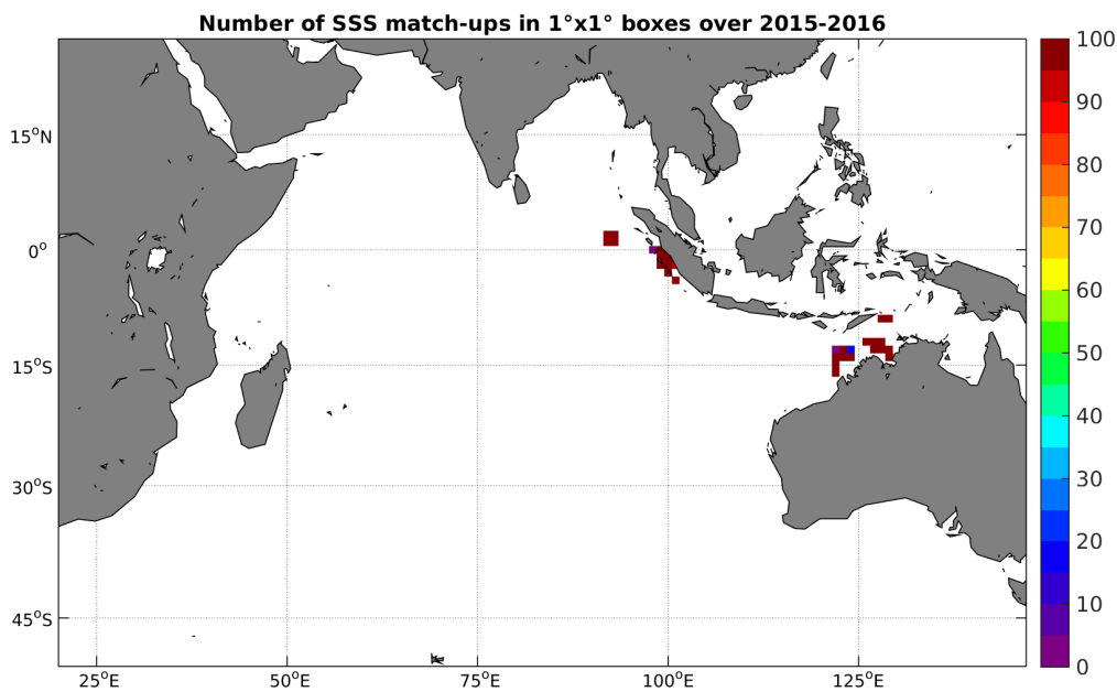
Figure 4: Number of SSS match-ups between TSG-SAMOS SSS and the SMAP-L2-JPL-V4 SSS product for the Indian Ocean Pi-MEP region over 1^\circ \times 1^\circ boxes and for the full satellite product period.
