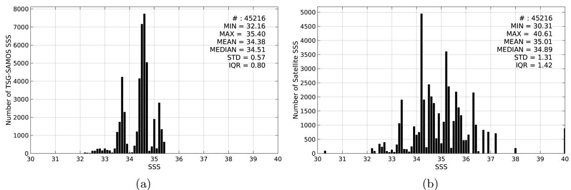
Figure 2: Histograms of SSS from TSG-SAMOS (a) and SMAP-L2-JPL-V4 (b) considering all match-up pairs per bins of 0.1 over the Indian Ocean Pi-MEP region and for the full satellite product period.
