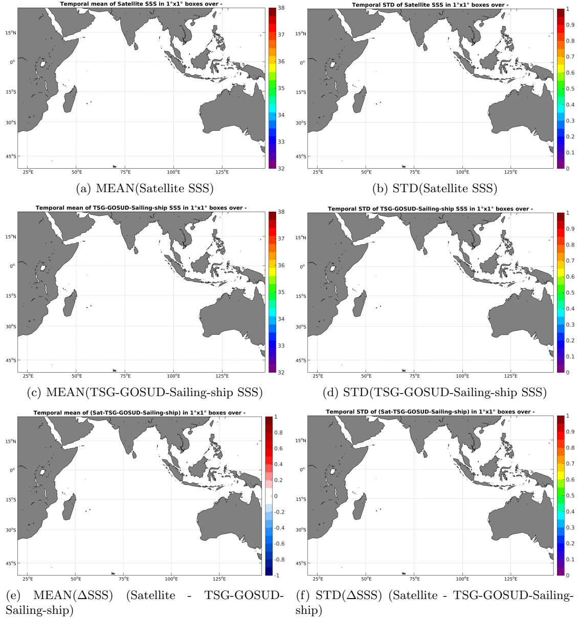
Figure 6: Temporal mean (left) and STD (right) of SSS from SMAP-L2-JPL-V4 (top), TSG-GOSUD-Sailing-ship (middle), and of \Delta SSS (Satellite - TSG-GOSUD-Sailing-ship). Only match-up pairs are used to generate these maps.
