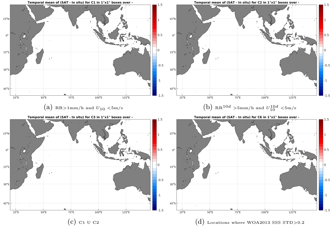
Figure 12: Temporal mean gridded over spatial boxes of size 1^\circ \times 1^\circ of \Delta SSS (SMAP-L2-JPL-V4 - TSG-GOSUD-Sailing-ship) for 4 different subdatasets corresponding to: RR > 1 mm/h and U_{10} < 5 m/s (a), RR^{10d} > 5 mm/h and U_{10}^{10d} < 5 m/s (b), C1 U C2 (c), Locations where WOA2013 SSS STD > 0.2 (d).
