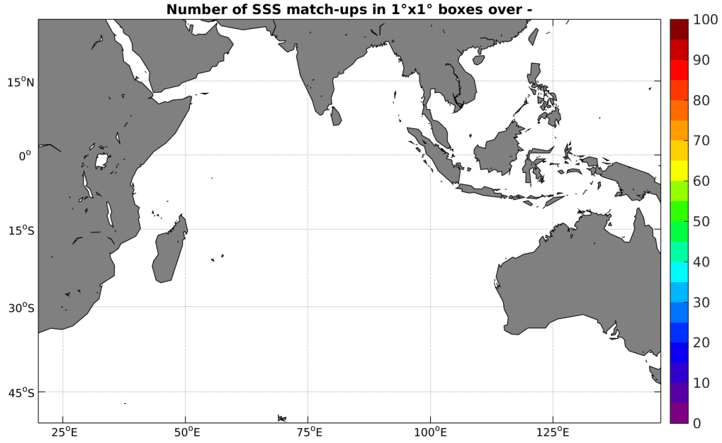
Figure 4: Number of SSS match-ups between TSG-GOSUD-Sailing-ship SSS and the SMAP-L2-JPL-V4 SSS product for the Indian Ocean Pi-MEP region over 1^\circ \times 1^\circ boxes and for the full satellite product period.
