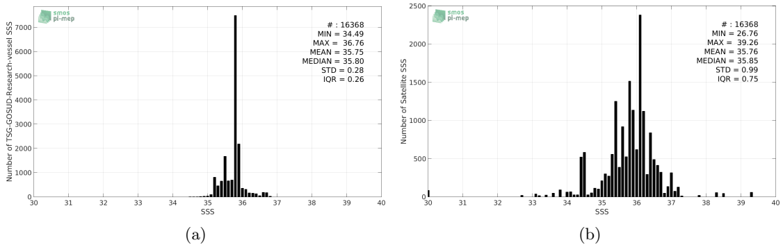
Figure 2: Histograms of SSS from TSG-GOSUD-Research-vessel (a) and SMAP-L2-JPL-V4 (b) considering all match-up pairs per bins of 0.1 over the Indian Ocean Pi-MEP region and for the full satellite product period.
