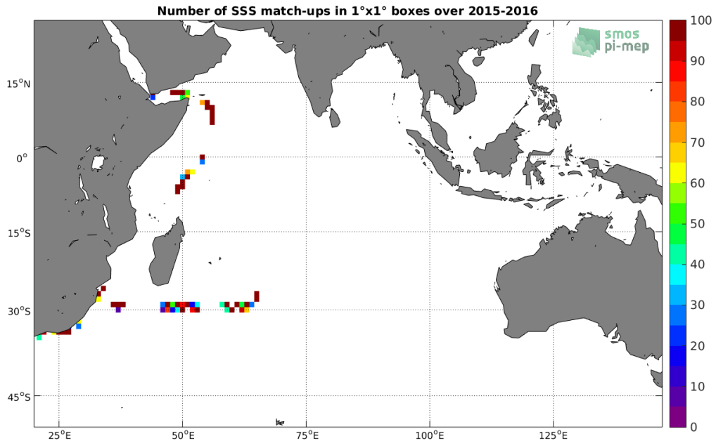
Figure 4: Number of SSS match-ups between TSG-GOSUD-Research-vessel SSS and the SMAP-L2-JPL-V4 SSS product for the Indian Ocean Pi-MEP region over 1°x1° boxes and for the full satellite product period.
