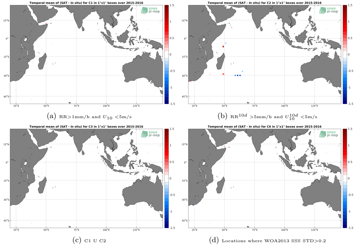
Figure 12: Temporal mean gridded over spatial boxes of size 1^\circ \times 1^\circ of \Delta SSS (SMAP-L2-JPL-V4 - TSG-GOSUD-Research-vessel) for 4 different subdatasets corresponding to: RR > 1\text{mm/h} and U_{10} < 5\text{m/s} (a), RR^{10d} > 5\text{mm/h} and U_{10}^{10d} < 5\text{m/s} (b), C1 U C2 (c), Locations where WOA2013 SSS STD > 0.2 (d).
