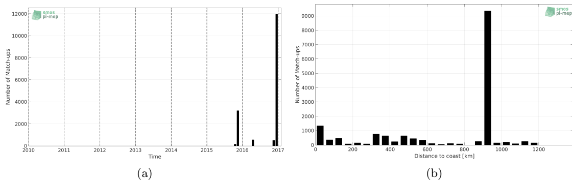
Figure 1: Number of match-ups between TSG-GOSUD-Research-vessel and SMAP-L2-JPL-V4 SSS as a function of time (a) and as function of the distance to coast (b) over the Indian Ocean Pi-MEP region and for the full satellite product period.
