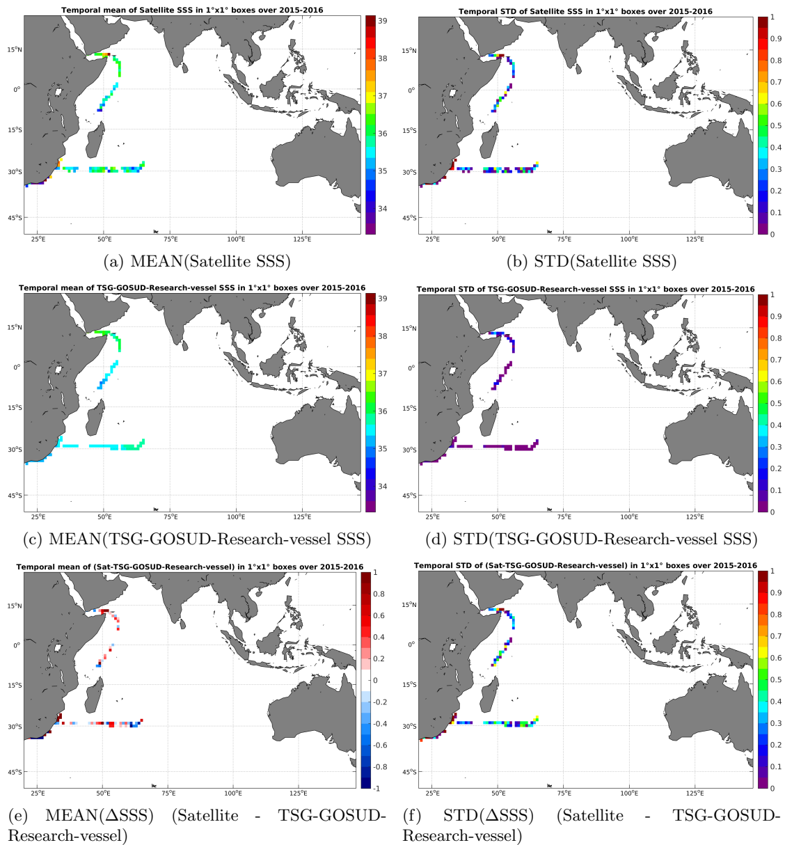
Figure 6: Temporal mean (left) and STD (right) of SSS from SMAP-L2-JPL-V4 (top), TSG-GOSUD-Research-vessel (middle), and of \Delta SSS (Satellite - TSG-GOSUD-Research-vessel). Only match-up pairs are used to generate these maps.
