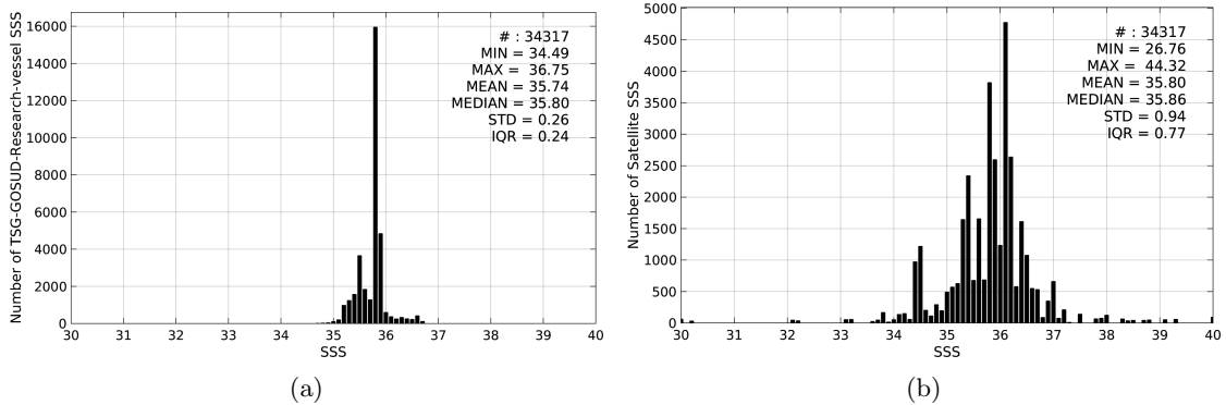
Figure 2: Histograms of SSS from TSG-GOSUD-Research-vessel (a) and SMAP-L2-JPL-V4 (b) considering all match-up pairs per bins of 0.1 over the Indian Ocean Pi-MEP region and for the full satellite product period.
