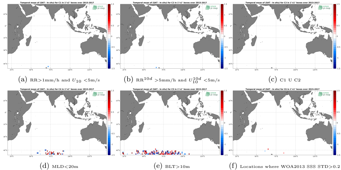
Figure 12: Temporal mean gridded over spatial boxes of size 1^\circ \times 1^\circ of \Delta\text{SSS} (SMAP-L2-JPL-V4 - Sea mammals) for 6 different subdatasets corresponding to: RR > 1\text{mm/h} and U_{10} < 5\text{m/s} (a), RR^{10d} > 5\text{mm/h} and U_{10}^{10d} < 5\text{m/s} (b), C1 U C2 (c), MLD < 20\text{m} (d), BLT > 10\text{m} (e), Locations where WOA2013 SSS STD > 0.2 (f).
