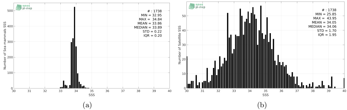
Figure 2: Histograms of SSS from Sea mammals (a) and SMAP-L2-JPL-V4 (b) considering all match-up pairs per bins of 0.1 over the Indian Ocean Pi-MEP region and for the full satellite product period.
