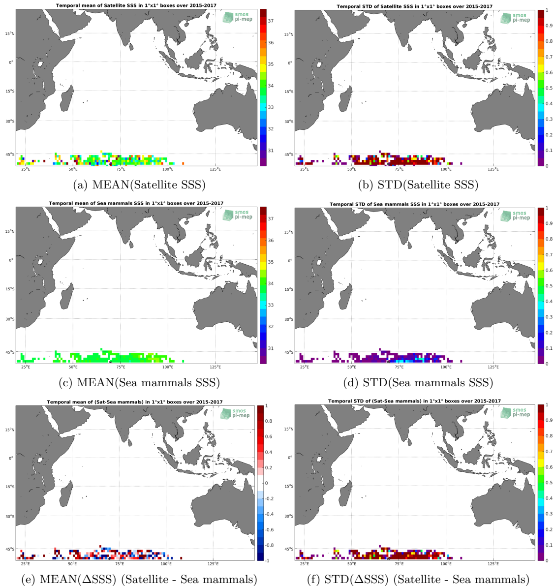
Figure 6: Temporal mean (left) and STD (right) of SSS from SMAP-L2-JPL-V4 (top), Sea mammals (middle), and of \Delta SSS (Satellite - Sea mammals). Only match-up pairs are used to generate these maps.
