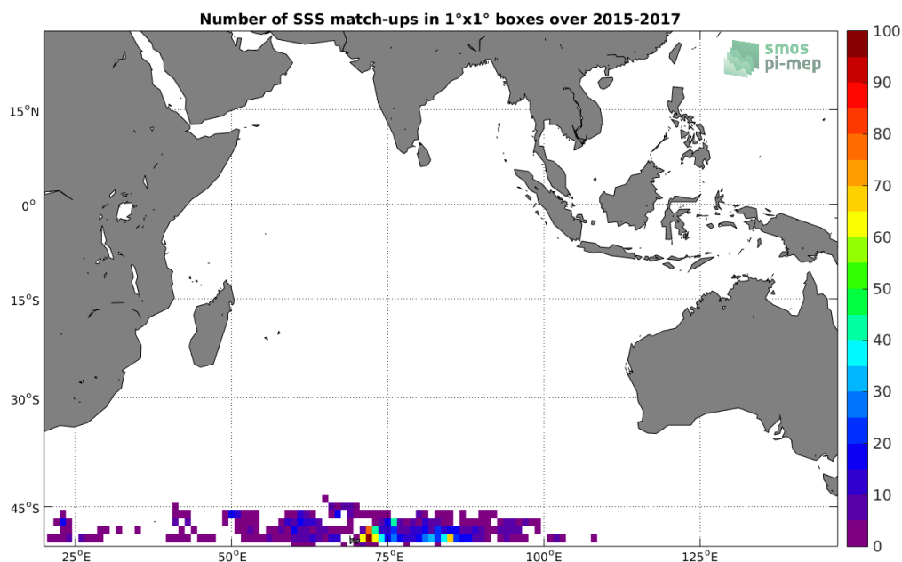
Figure 4: Number of SSS match-ups between Sea mammals SSS and the SMAP-L2-JPL-V4 SSS product for the Indian Ocean Pi-MEP region over 1°x1° boxes and for the full satellite product period.
