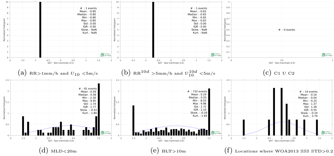
Figure 13: Normalized histogram of \Delta\text{SSS} (SMAP-L2-JPL-V4 - Sea mammals) for 6 different sub-datasets corresponding to: RR > 1\text{mm/h} and U_{10} < 5\text{m/s} (a), RR^{10d} > 5\text{mm/h} and U_{10}^{10d} < 5\text{m/s} (b), C1 U C2 (c), MLD < 20\text{m} (d), BLT > 10\text{m} (e), Locations where WOA2013 SSS STD > 0.2 (f).
