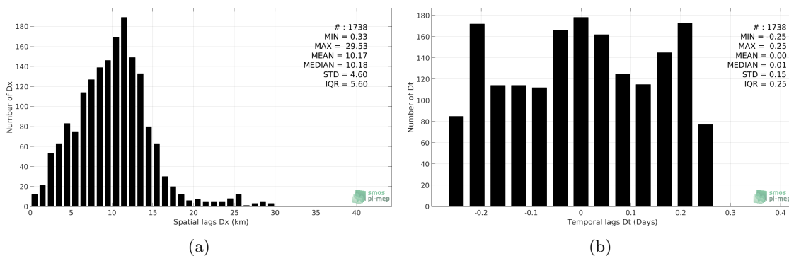
Figure 5: Histograms of the spatial (a) and temporal (b) lags between the time of the Sea mammals measurements and the date of the corresponding SMAP-L2-JPL-V4 SSS product.
