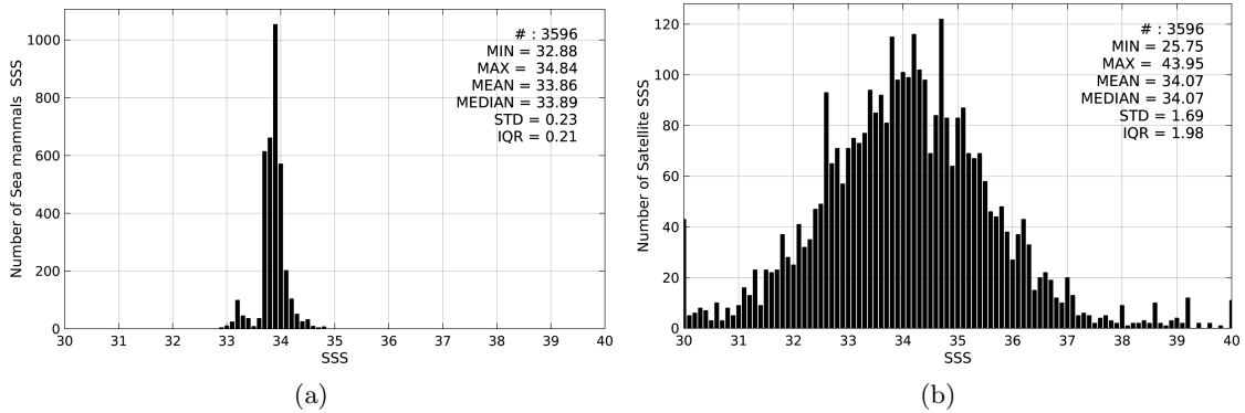
Figure 2: Histograms of SSS from Sea mammals (a) and SMAP-L2-JPL-V4 (b) considering all match-up pairs per bins of 0.1 over the Indian Ocean Pi-MEP region and for the full satellite product period.
