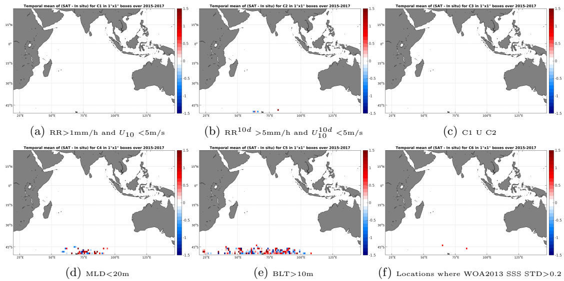
Figure 12: Temporal mean gridded over spatial boxes of size 1^\circ \times 1^\circ of \Delta SSS (SMAP-L2-JPL-V4 - Sea mammals) for 6 different subdatasets corresponding to: RR > 1\text{mm/h} and U_{10} < 5\text{m/s} (a), RR^{10d} > 5\text{mm/h} and U_{10}^{10d} < 5\text{m/s} (b), C1 U C2 (c), MLD < 20\text{m} (d), BLT > 10\text{m} (e), Locations where WOA2013 SSS STD > 0.2 (f).
