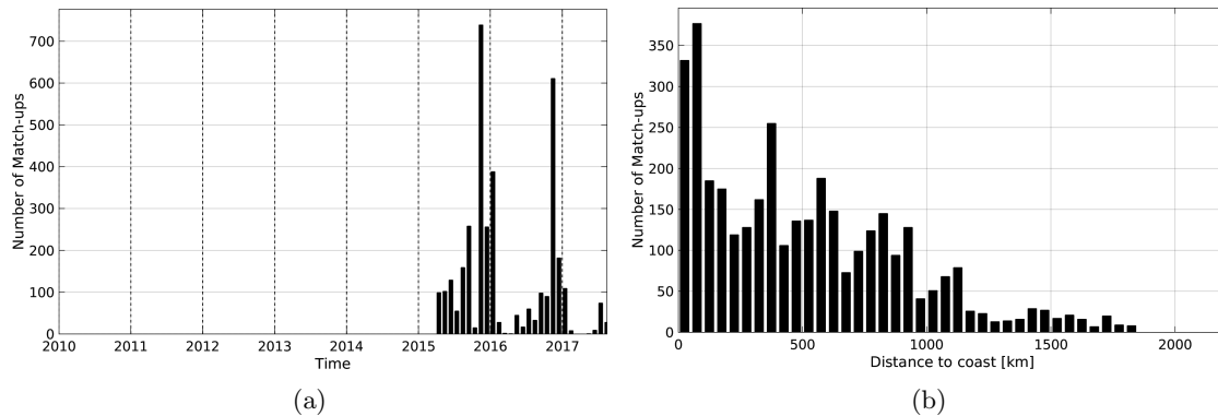
Figure 1: Number of match-ups between Sea mammals and SMAP-L2-JPL-V4 SSS as a function of time (a) and as function of the distance to coast (b) over the Indian Ocean Pi-MEP region and for the full satellite product period.
