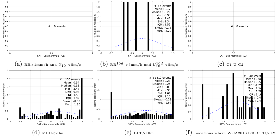
Figure 13: Normalized histogram of \Delta SSS (SMAP-L2-JPL-V4 - Sea mammals) for 6 different sub-datasets corresponding to: RR > 1mm/h and U_{10} < 5 m/s (a), RR 10d > 5mm/h and U_{10}^{10d} < 5 m/s (b), C1 U C2 (c), MLD < 20m (d), BLT > 10m (e), Locations where WOA2013 SSS STD > 0.2 (f).
