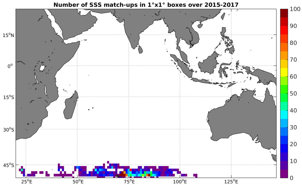
Figure 4: Number of SSS match-ups between Sea mammals SSS and the SMAP-L2-JPL-V4 SSS product for the Indian Ocean Pi-MEP region over 1^\circ \times 1^\circ boxes and for the full satellite product period.
