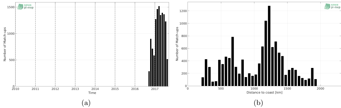
Figure 1: Number of match-ups between Surface drifters and SMAP-L2-JPL-V4 SSS as a function of time (a) and as function of the distance to coast (b) over the Indian Ocean Pi-MEP region and for the full satellite product period.
