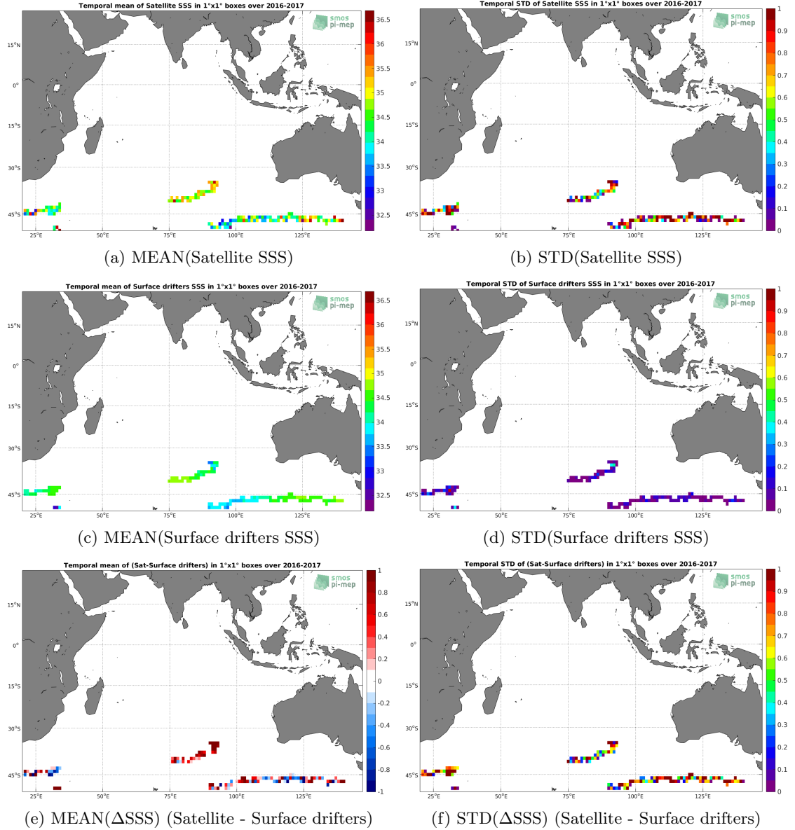
Figure 5: Temporal mean (left) and STD (right) of SSS from SMAP-L2-JPL-V4 (top), Surface drifters (middle), and of \Delta SSS (Satellite - Surface drifters). Only match-up pairs are used to generate these maps.
