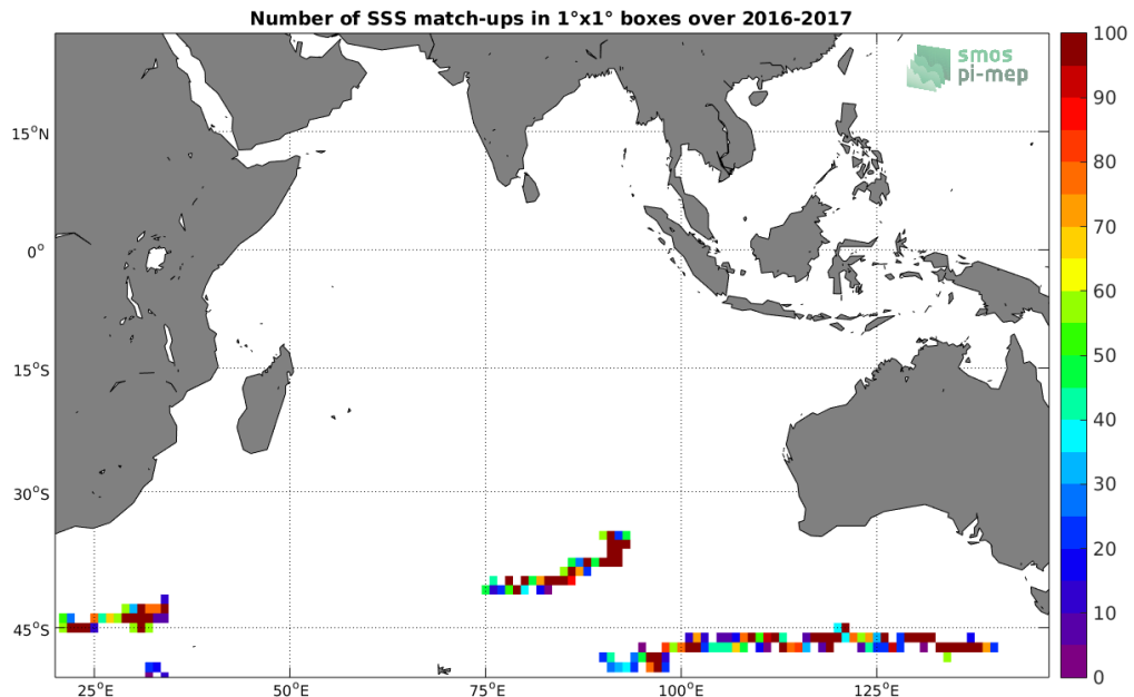
Figure 3: Number of SSS match-ups between Surface drifters SSS and the SMAP-L2-JPL-V4 SSS product for the Indian Ocean Pi-MEP region over 1°x1° boxes and for the full satellite product period.
