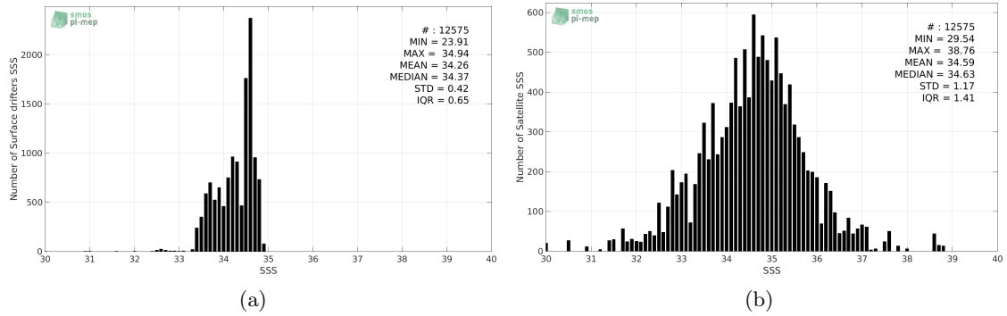
Figure 2: Histograms of SSS from Surface drifters (a) and SMAP-L2-JPL-V4 (b) considering all match-up pairs per bins of 0.1 over the Indian Ocean Pi-MEP region and for the full satellite product period.
