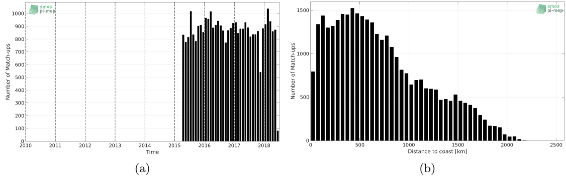
Figure 1: Number of match-ups between Argo and SMAP-L2-JPL-V4 SSS as a function of time (a) and as function of the distance to coast (b) over the Indian Ocean Pi-MEP region and for the full satellite product period.
