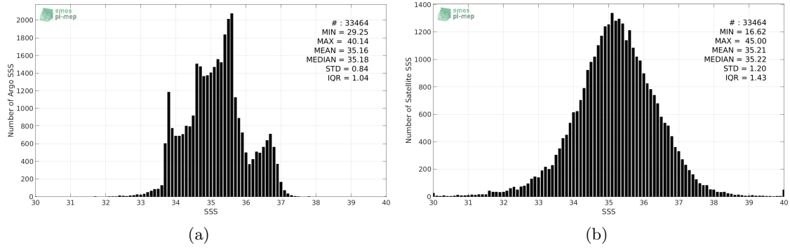
Figure 2: Histograms of SSS from Argo (a) and SMAP-L2-JPL-V4 (b) considering all match-up pairs per bins of 0.1 over the Indian Ocean Pi-MEP region and for the full satellite product period.
