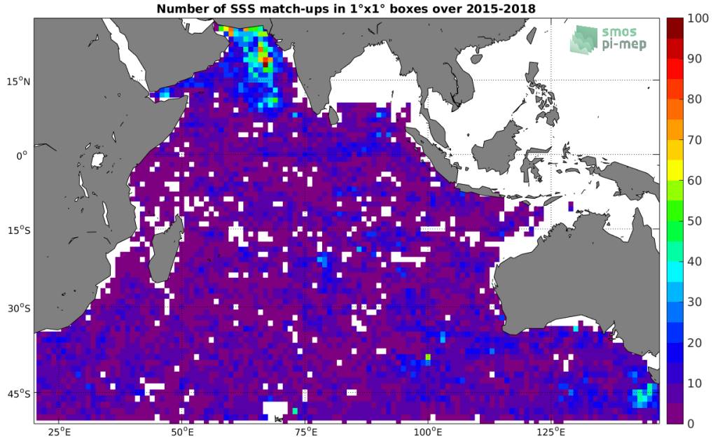
Figure 4: Number of SSS match-ups between Argo SSS and the SMAP-L2-JPL-V4 SSS product for the Indian Ocean Pi-MEP region over 1^\circ \times 1^\circ boxes and for the full satellite product period.
