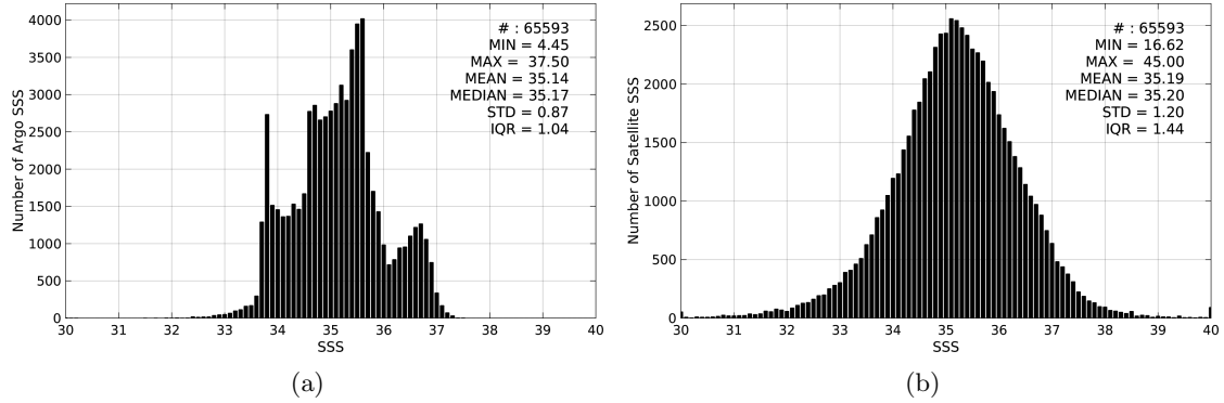
Figure 2: Histograms of SSS from Argo (a) and SMAP-L2-JPL-V4 (b) considering all match-up pairs per bins of 0.1 over the Indian Ocean Pi-MEP region and for the full satellite product period.
