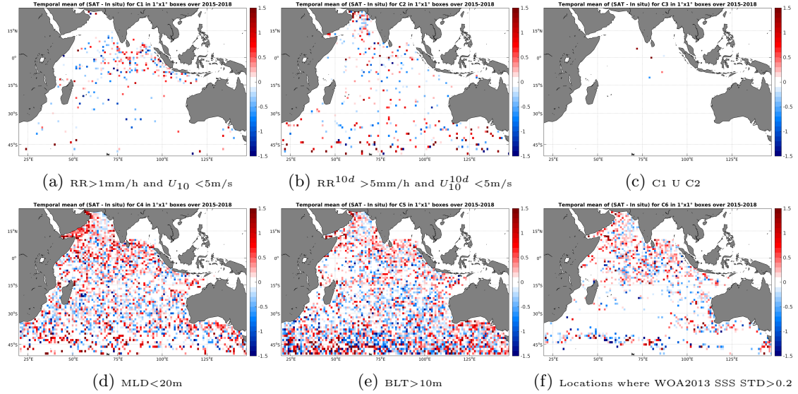
Figure 12: Temporal mean gridded over spatial boxes of size 1^\circ \times 1^\circ of \Delta\text{SSS} (SMAP-L2-JPL-V4 - Argo) for 6 different subdatasets corresponding to: \text{RR} > 1\text{mm/h} and U_{10} < 5\text{m/s} (a), \text{RR}^{10d} > 5\text{mm/h} and U_{10}^{10d} < 5\text{m/s} (b), C1 U C2 (c), \text{MLD} < 20\text{m} (d), \text{BLT} > 10\text{m} (e), Locations where WOA2013 SSS STD > 0.2 (f).
