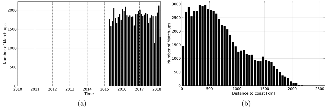
Figure 1: Number of match-ups between Argo and SMAP-L2-JPL-V4 SSS as a function of time (a) and as function of the distance to coast (b) over the Indian Ocean Pi-MEP region and for the full satellite product period.
