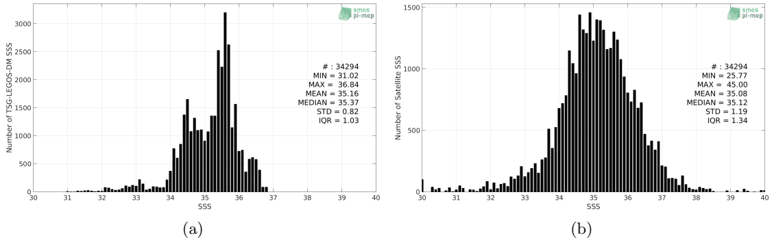
Figure 2: Histograms of SSS from TSG-LEGOS-DM (a) and SMAP-L2-JPL-V4.3 (b) considering all match-up pairs per bins of 0.1 over the Indian Ocean Pi-MEP region and for the full satellite product period.
