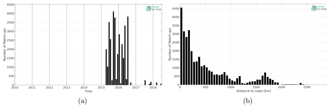
Figure 1: Number of match-ups between TSG-LEGOS-DM and SMAP-L2-JPL-V4.3 SSS as a function of time (a) and as function of the distance to coast (b) over the Indian Ocean Pi-MEP region and for the full satellite product period.
