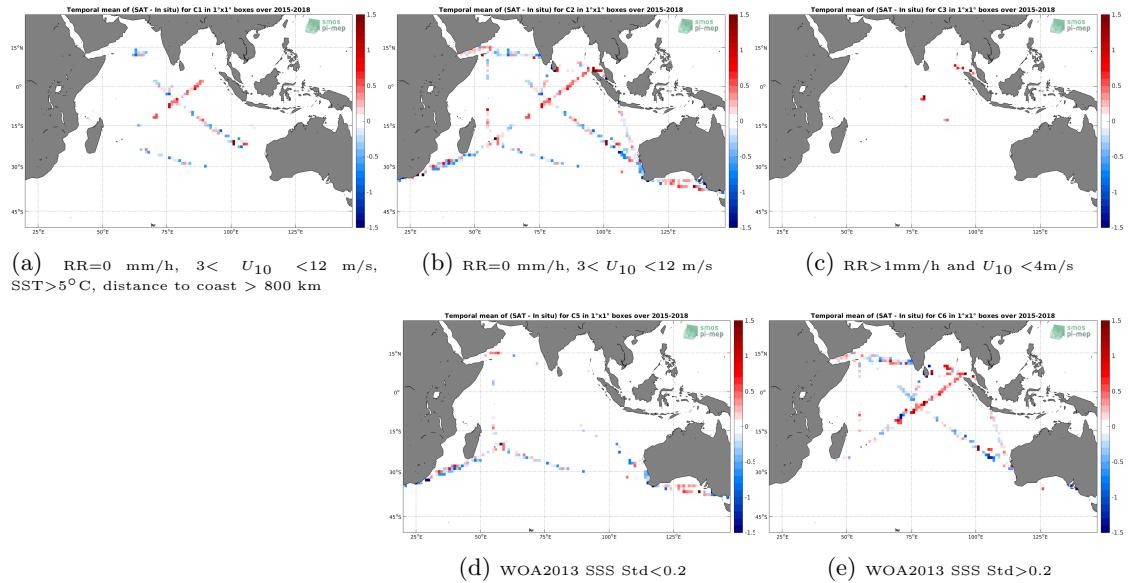
Figure 12: Temporal mean gridded over spatial boxes of size 1^\circ \times 1^\circ of \Delta SSS (SMAP-L2-JPL-V4.3 - TSG-LEGOS-DM) for 5 different subdatasets corresponding to:RR=0 mm/h, 3 < U_{10} < 12 m/s, SST >5^\circ C, distance to coast > 800 km (a), RR=0 mm/h, 3 < U_{10} < 12 m/s (b), RR >1 mm/h and U_{10} < 4 m/s (c), WOA2013 SSS Std <0.2 (d), WOA2013 SSS Std >0.2 (e).
