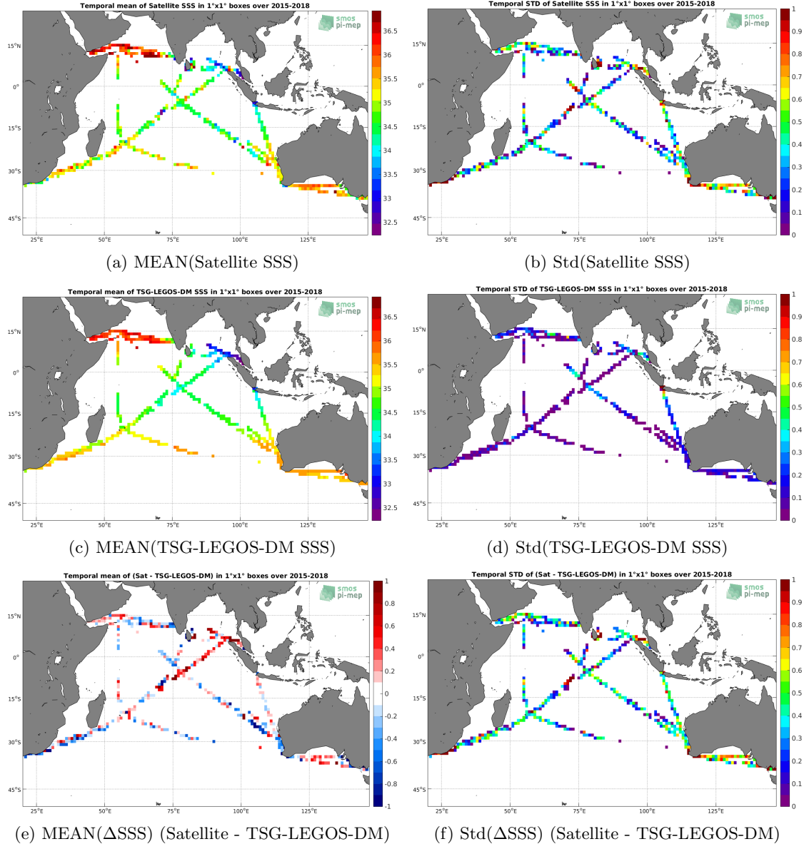
Figure 6: Temporal mean (left) and Std (right) of SSS from SMAP-L2-JPL-V4.3 (top), TSG-LEGOS-DM (middle), and of \Delta SSS (Satellite - TSG-LEGOS-DM). Only match-up pairs are used to generate these maps.
