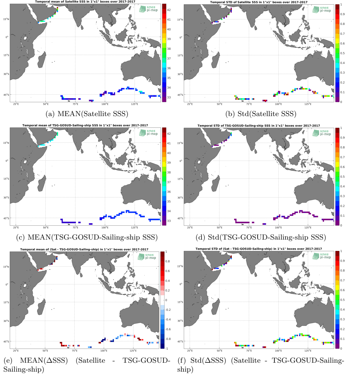
Figure 6: Temporal mean (left) and Std (right) of SSS from SMAP-L2-JPL-V4.3 (top), TSG-GOSUD-Sailing-ship (middle), and of \Delta SSS (Satellite - TSG-GOSUD-Sailing-ship). Only match-up pairs are used to generate these maps.
