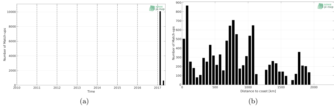
Figure 1: Number of match-ups between TSG-GOSUD-Sailing-ship and SMAP-L2-JPL-V4.3 SSS as a function of time (a) and as function of the distance to coast (b) over the Indian Ocean Pi-MEP region and for the full satellite product period.
