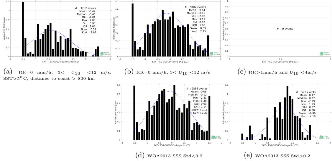
Figure 13: Normalized histogram of \Delta SSS (SMAP-L2-JPL-V4.3 - TSG-GOSUD-Sailing-ship) for 5 different subdatasets corresponding to: RR=0 mm/h, 3 < U_{10} < 12 m/s, SST > 5^\circ\text{C} , distance to coast > 800 km (a), RR=0 mm/h, 3 < U_{10} < 12 m/s (b), RR > 1\text{mm/h} and U_{10} < 4\text{m/s} (c), WOA2013 SSS Std < 0.2 (d), WOA2013 SSS Std > 0.2 (e).
