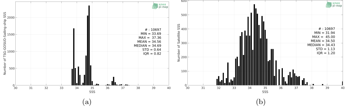
Figure 2: Histograms of SSS from TSG-GOSUD-Sailing-ship (a) and SMAP-L2-JPL-V4.3 (b) considering all match-up pairs per bins of 0.1 over the Indian Ocean Pi-MEP region and for the full satellite product period.
