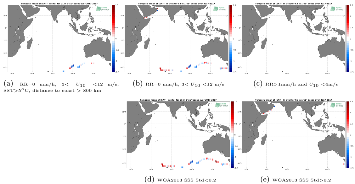
Figure 12: Temporal mean gridded over spatial boxes of size 1^\circ \times 1^\circ of \Delta SSS (SMAP-L2-JPL-V4.2 - TSG-GOSUD-Sailing-ship) for 5 different subdatasets corresponding to:RR=0 mm/h, 3 < U_{10} < 12 m/s, SST >5^\circ C, distance to coast > 800 km (a), RR=0 mm/h, 3 < U_{10} < 12 m/s (b), RR >1 mm/h and U_{10} < 4 m/s (c), WOA2013 SSS Std <0.2 (d), WOA2013 SSS Std >0.2 (e).
