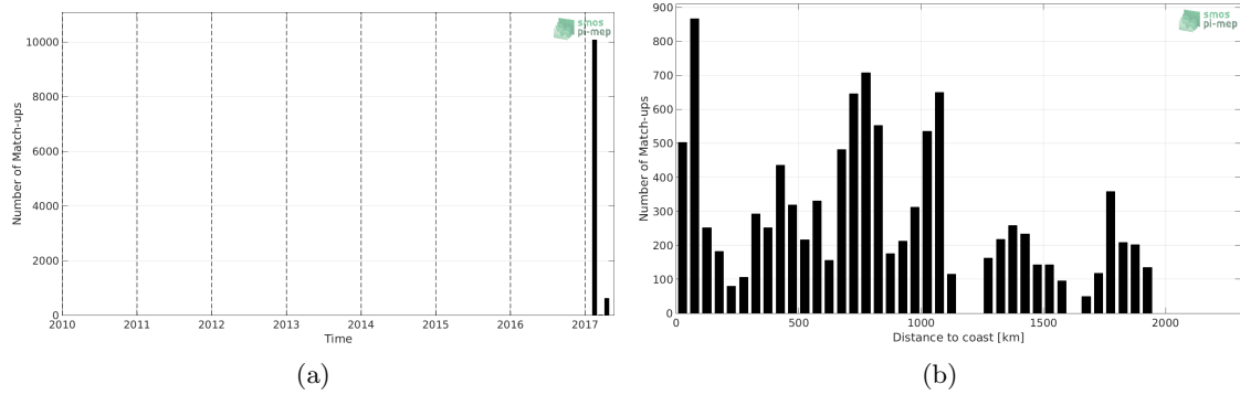
Figure 1: Number of match-ups between TSG-GOSUD-Sailing-ship and SMAP-L2-JPL-V4.2 SSS as a function of time (a) and as function of the distance to coast (b) over the Indian Ocean Pi-MEP region and for the full satellite product period.
