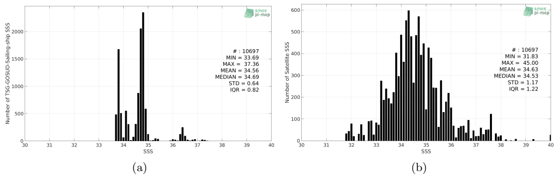
Figure 2: Histograms of SSS from TSG-GOSUD-Sailing-ship (a) and SMAP-L2-JPL-V4.2 (b) considering all match-up pairs per bins of 0.1 over the Indian Ocean Pi-MEP region and for the full satellite product period.
