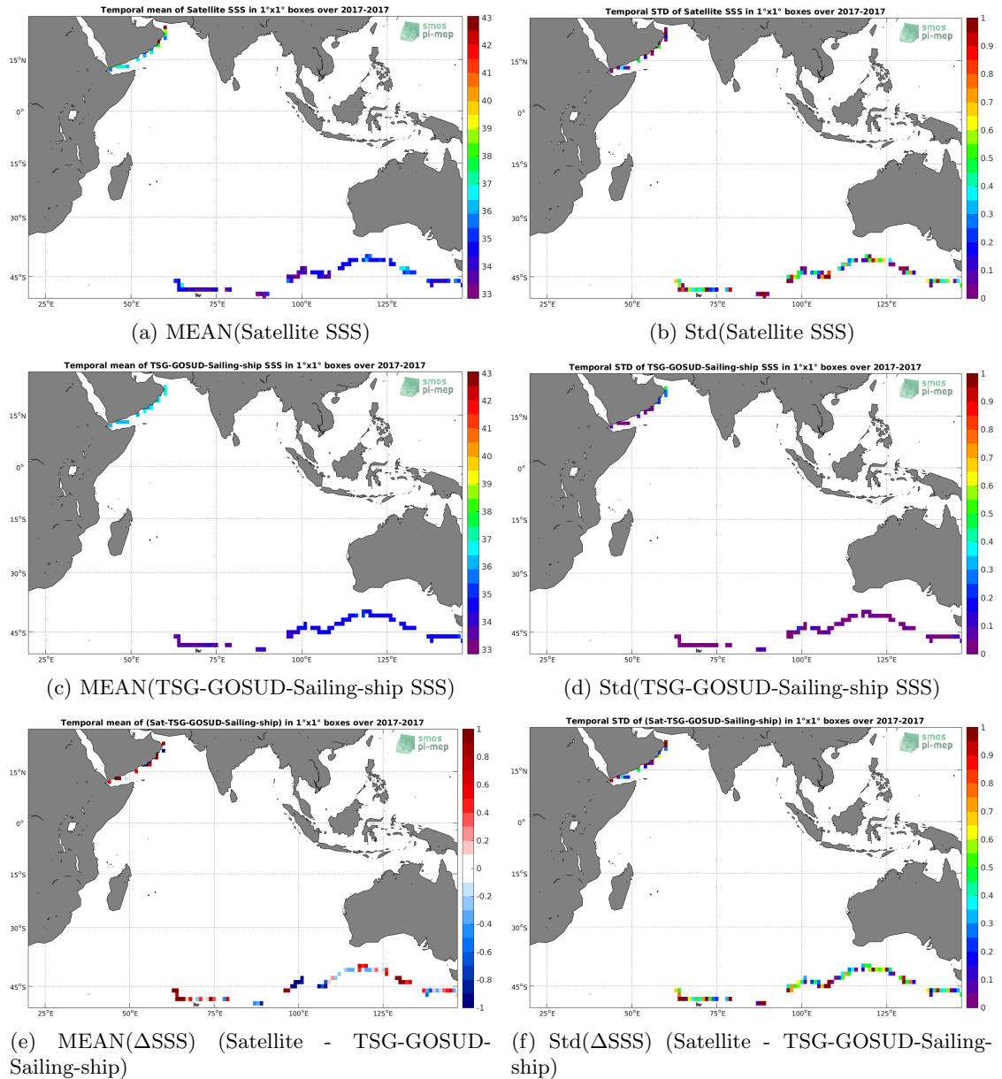
Figure 6: Temporal mean (left) and Std (right) of SSS from SMAP-L2-JPL-V4.2 (top), TSG-GOSUD-Sailing-ship (middle), and of \Delta SSS (Satellite - TSG-GOSUD-Sailing-ship). Only match-up pairs are used to generate these maps.
