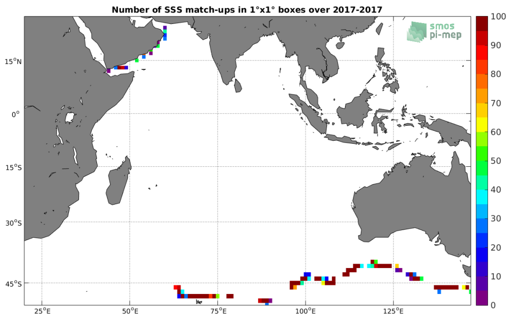
Figure 4: Number of SSS match-ups between TSG-GOSUD-Sailing-ship SSS and the SMAP-L2-JPL-V4.2 SSS product for the Indian Ocean Pi-MEP region over 1^{\circ} \times 1^{\circ} boxes and for the full satellite product period.
