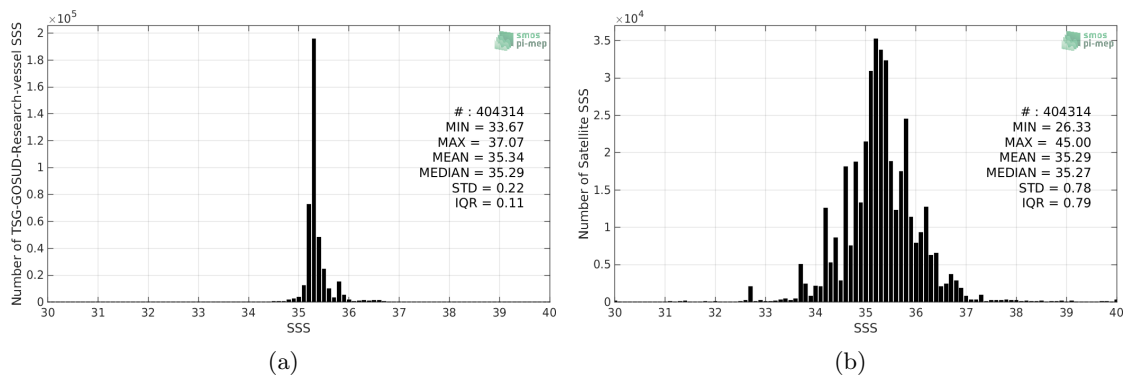
Figure 2: Histograms of SSS from TSG-GOSUD-Research-vessel (a) and SMAP-L2-JPL-V4.2 (b) considering all match-up pairs per bins of 0.1 over the Indian Ocean Pi-MEP region and for the full satellite product period.
