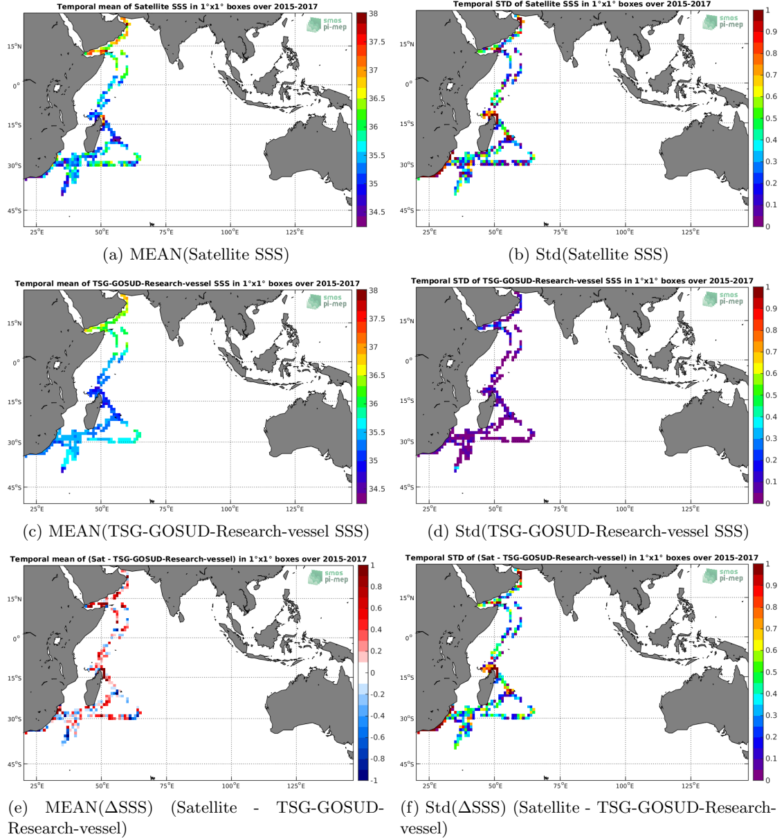
Figure 6: Temporal mean (left) and Std (right) of SSS from SMAP-L2-JPL-V4.2 (top), TSG-GOSUD-Research-vessel (middle), and of \Delta SSS (Satellite - TSG-GOSUD-Research-vessel). Only match-up pairs are used to generate these maps.
