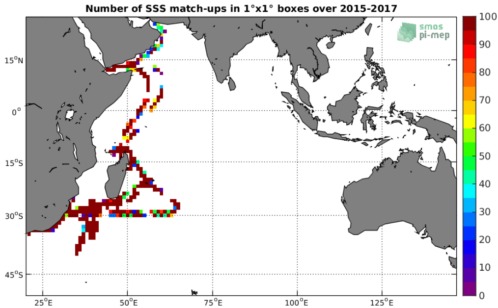
Figure 4: Number of SSS match-ups between TSG-GOSUD-Research-vessel SSS and the SMAP-L2-JPL-V4.2 SSS product for the Indian Ocean Pi-MEP region over 1^\circ \times 1^\circ boxes and for the full satellite product period.
