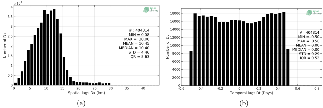
Figure 5: Histograms of the spatial (a) and temporal (b) lags between the time of the TSG-GOSUD-Research-vessel measurements and the date of the corresponding SMAP-L2-JPL-V4.2 SSS product.
