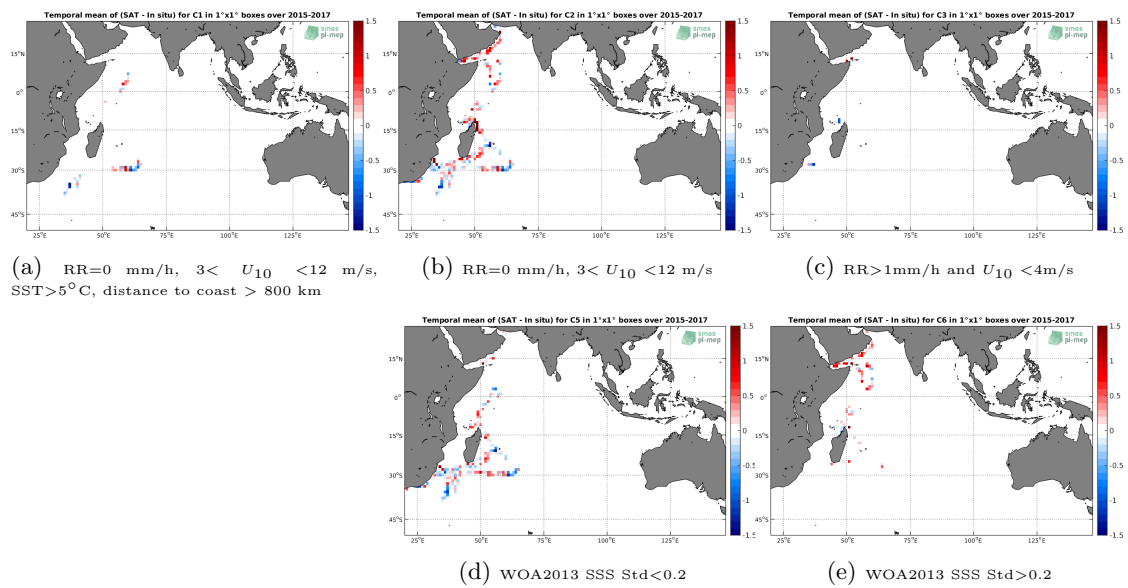
Figure 12: Temporal mean gridded over spatial boxes of size 1^\circ \times 1^\circ of \Delta SSS (SMAP-L2-JPL-V4.2 - TSG-GOSUD-Research-vessel) for 5 different subdatasets corresponding to:RR=0 mm/h, 3 < U_{10} < 12 m/s, SST >5^\circ C, distance to coast > 800 km (a), RR=0 mm/h, 3 < U_{10} < 12 m/s (b), RR >1 mm/h and U_{10} < 4 m/s (c), WOA2013 SSS Std <0.2 (d), WOA2013 SSS Std >0.2 (e).
