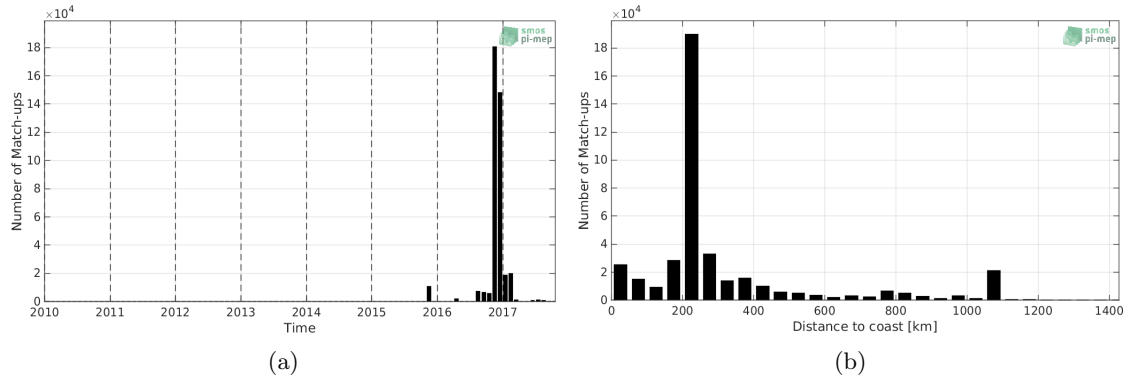
Figure 1: Number of match-ups between TSG-GOSUD-Research-vessel and SMAP-L2-JPL-V4.2 SSS as a function of time (a) and as function of the distance to coast (b) over the Indian Ocean Pi-MEP region and for the full satellite product period.
