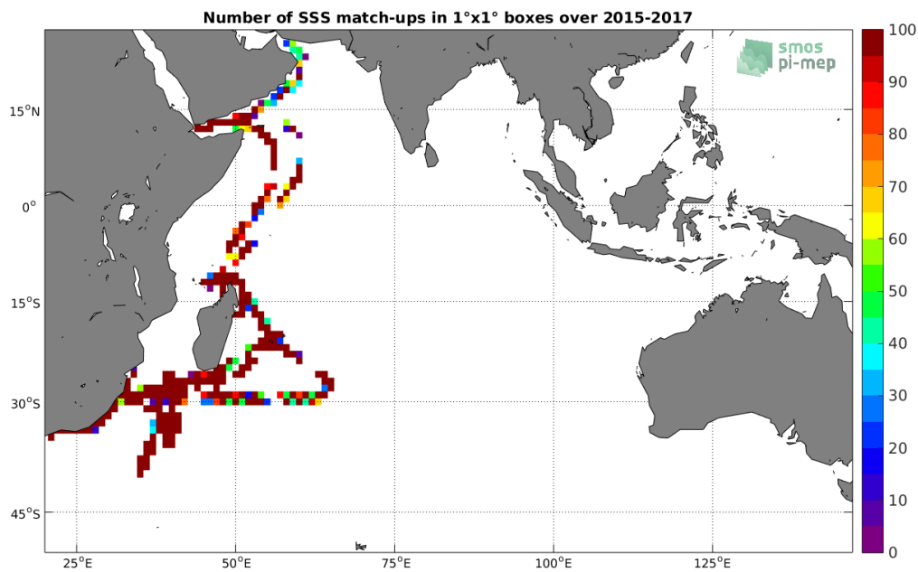
Figure 4: Number of SSS match-ups between TSG-GOSUD-Research-vessel SSS and the SMAP-L2-JPL-V4.2 SSS product for the Indian Ocean Pi-MEP region over 1^\circ \times 1^\circ boxes and for the full satellite product period.
