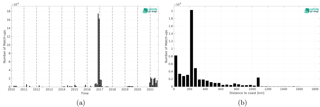
Figure 2: Number of match-ups between TSG (GOSUD-Research-vessel) and ISAS SSS as a function of time (a) and as function of the distance to coast (b) over the Indian Ocean Pi-MEP region and for the full satellite product period.
