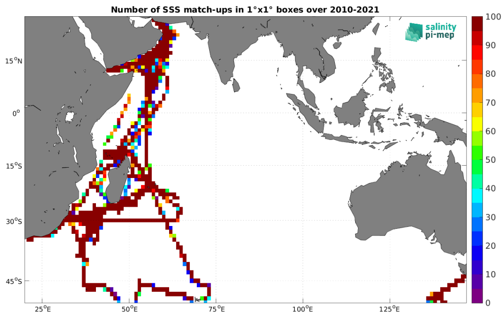
Figure 5: Number of SSS match-ups between TSG (GOSUD-Research-vessel) SSS and the ISAS SSS product for the Indian Ocean Pi-MEP region over 1^\circ \times 1^\circ boxes and for the full satellite product period.
