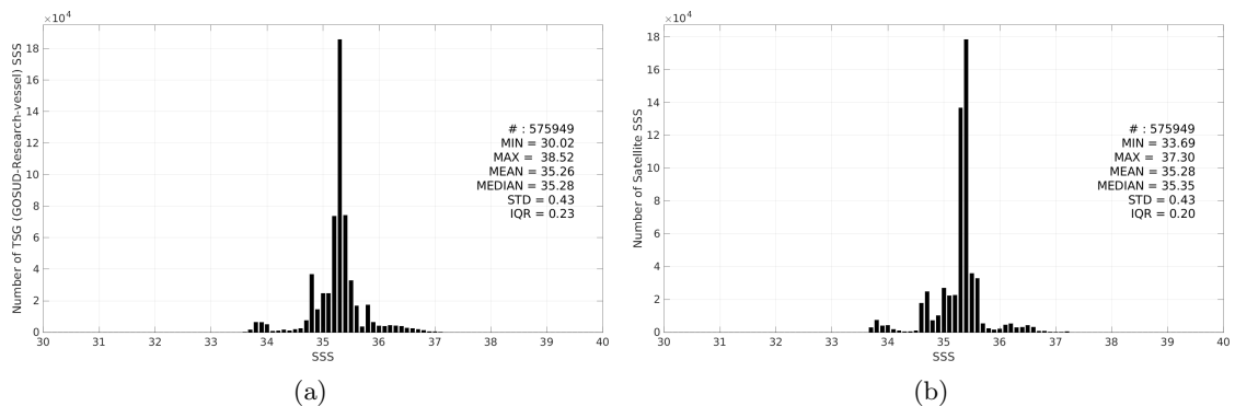
Figure 3: Histograms of SSS from TSG (GOSUD-Research-vessel) (a) and ISAS (b) considering all match-up pairs per bins of 0.1 over the Indian Ocean Pi-MEP region and for the full satellite product period.
