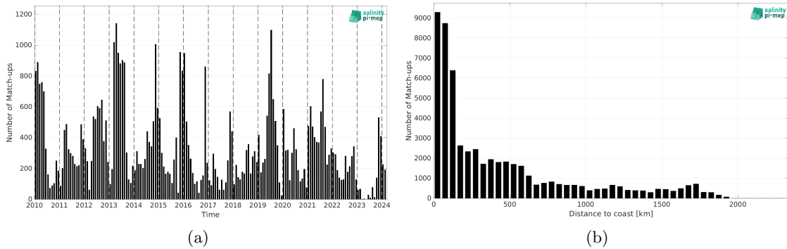
Figure 2: Number of match-ups between Marine mammals and ISAS v7 - Monthly (Ifremer-LOPS-CMEMS) SSS as a function of time (a) and as function of the distance to coast (b) over the Indian Ocean Pi-MEP region and for the full satellite product period.
