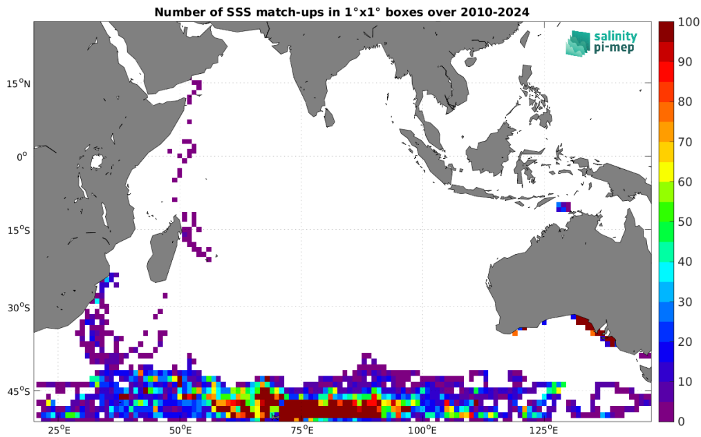
Figure 5: Number of SSS match-ups between Marine mammals SSS and the ISAS v7 - Monthly (Ifremer-LOPS-CMEMS) SSS product for the Indian Ocean Pi-MEP region over 1^{\circ} \times 1^{\circ} boxes and for the full satellite product period.
