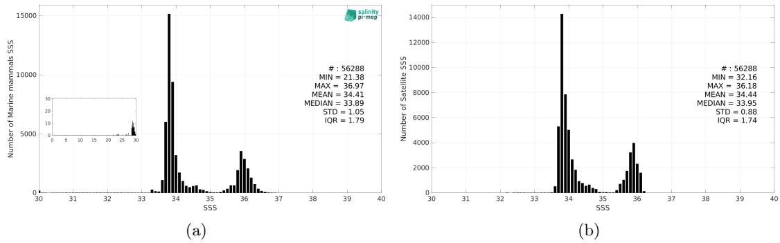
Figure 3: Histograms of SSS from Marine mammals (a) and ISAS v7 - Monthly (Ifremer-LOPS-CMEMS) (b) considering all match-up pairs per bins of 0.1 over the Indian Ocean Pi-MEP region and for the full satellite product period.
