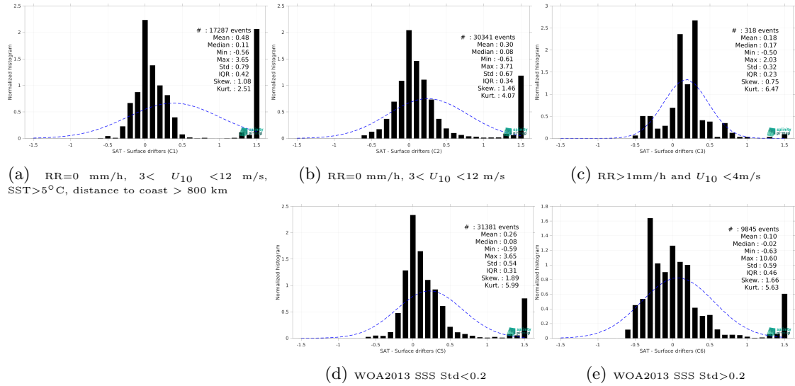
Figure 14: Normalized histogram of \Delta\text{SSS} (ISAS v7 - Monthly (Ifremer-LOPS-CMEMS) - Surface drifters) for 5 different subdatasets corresponding to: RR=0 mm/h, 3 < U_{10} < 12 m/s, SST > 5^\circ\text{C} , distance to coast > 800 km (a), RR=0 mm/h, 3 < U_{10} < 12 m/s (b), RR > 1 mm/h and U_{10} < 4 m/s (c), WOA2013 SSS Std < 0.2 (d), WOA2013 SSS Std > 0.2 (e).
