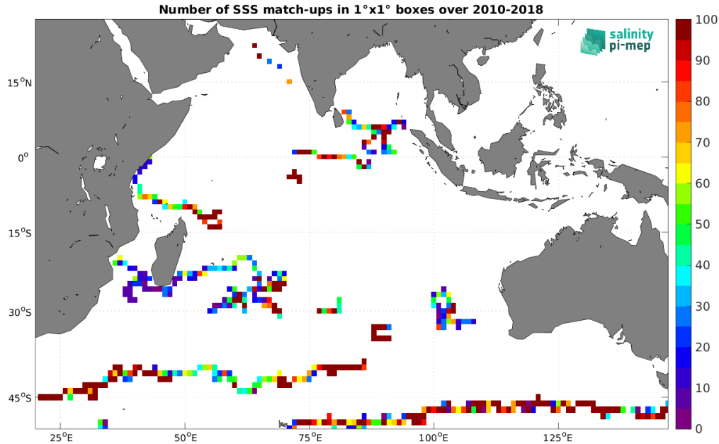
Figure 4: Number of SSS match-ups between Surface drifters SSS and the ISAS v7 - Monthly (Ifremer-LOPS-CMEMS) SSS product for the Indian Ocean Pi-MEP region over 1^\circ \times 1^\circ boxes and for the full satellite product period.
