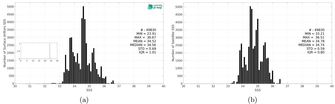
Figure 3: Histograms of SSS from Surface drifters (a) and ISAS v7 - Monthly (Ifremer-LOPS-CMEMS) (b) considering all match-up pairs per bins of 0.1 over the Indian Ocean Pi-MEP region and for the full satellite product period.
