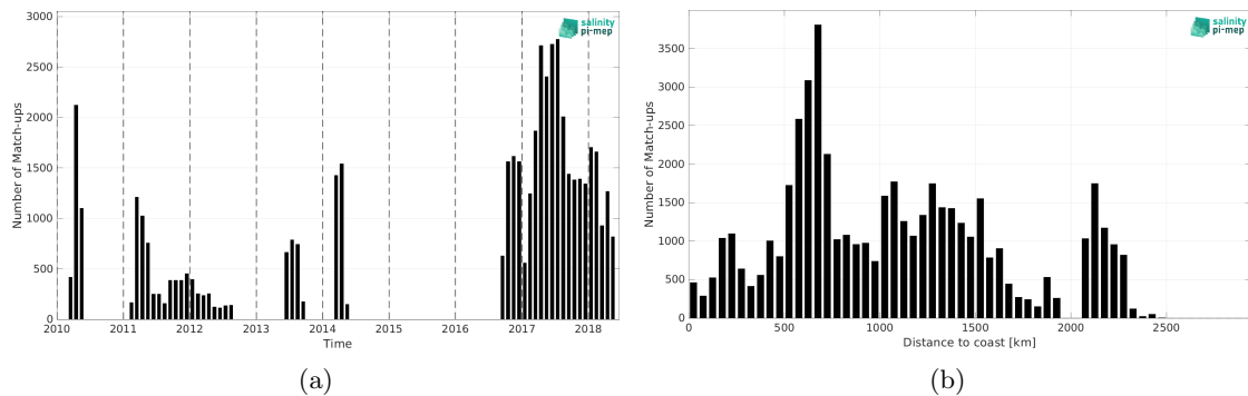
Figure 2: Number of match-ups between Surface drifters and ISAS SSS as a function of time (a) and as function of the distance to coast (b) over the Indian Ocean Pi-MEP region and for the full satellite product period.
