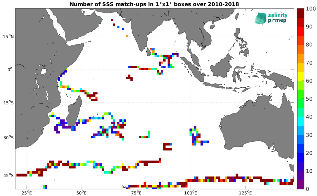
Figure 4: Number of SSS match-ups between Surface drifters SSS and the ISAS SSS product for the Indian Ocean Pi-MEP region over 1^\circ \times 1^\circ boxes and for the full satellite product period.
