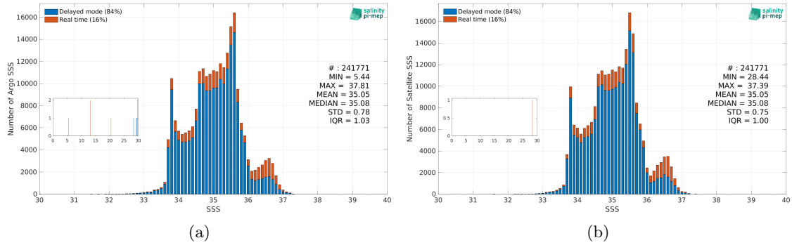
Figure 3: Histograms of SSS from Argo (a) and ISAS v7 - Monthly (Ifremer-LOPS-CMEMS) (b) considering all match-up pairs per bins of 0.1 over the Indian Ocean Pi-MEP region and for the full satellite product period.
