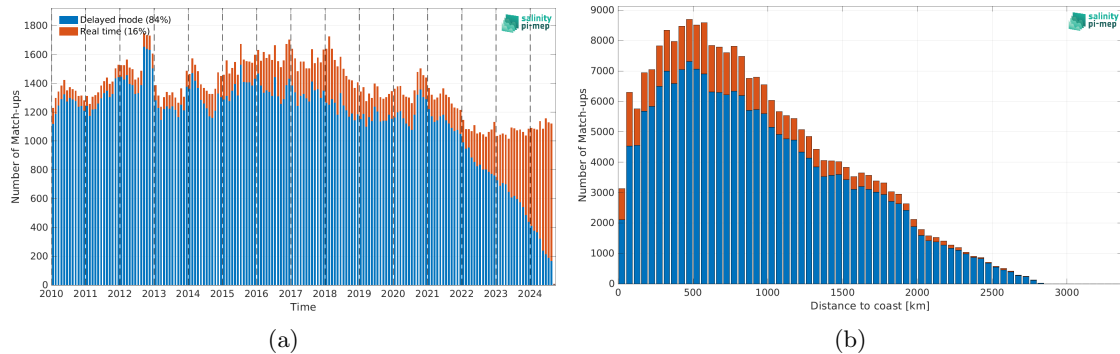
Figure 2: Number of match-ups between Argo and ISAS v7 - Monthly (Ifremer-LOPS-CMEMS) SSS as a function of time (a) and as function of the distance to coast (b) over the Indian Ocean Pi-MEP region and for the full satellite product period.
