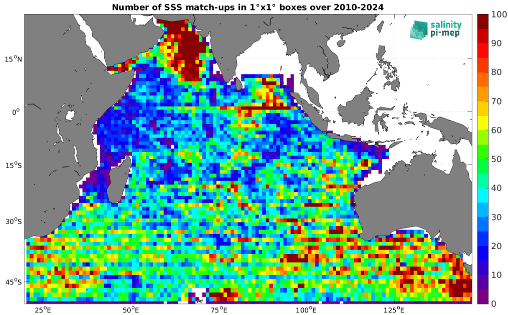
Figure 5: Number of SSS match-ups between Argo SSS and the ISAS v7 - Monthly (Ifremer-LOPS-CMEMS) SSS product for the Indian Ocean Pi-MEP region over 1^\circ \times 1^\circ boxes and for the full satellite product period.
