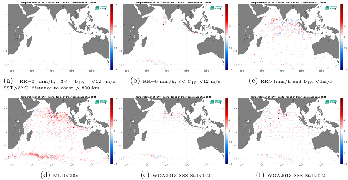
Figure 14: Temporal mean gridded over spatial boxes of size 1^\circ \times 1^\circ of \Delta\text{SSS} (ISAS v7 - Monthly (Ifremer-LOPS-CMEMS) - Argo) for 6 different subdatasets corresponding to:RR=0 mm/h, 3 < U_{10} < 12 m/s, SST > 5°C, distance to coast > 800 km (a), RR=0 mm/h, 3 < U_{10} < 12 m/s (b), RR > 1mm/h and U_{10} < 4 m/s (c),MLD < 20m (d),WOA2013 SSS Std < 0.2 (e),WOA2013 SSS Std > 0.2 (f).
