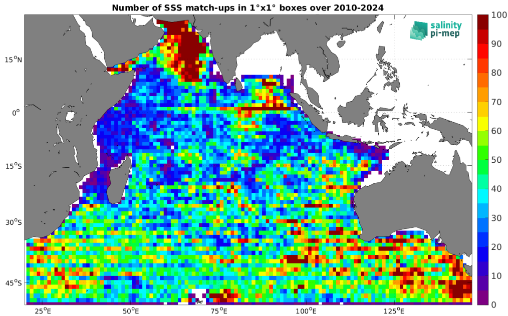
Figure 5: Number of SSS match-ups between Argo SSS and the ISAS SSS product for the Indian Ocean Pi-MEP region over 1^\circ \times 1^\circ boxes and for the full satellite product period.
