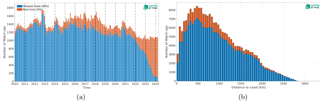
Figure 2: Number of match-ups between Argo and ISAS SSS as a function of time (a) and as function of the distance to coast (b) over the Indian Ocean Pi-MEP region and for the full satellite product period.
