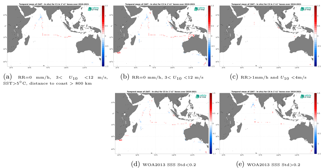
Figure 14: Temporal mean gridded over spatial boxes of size 1^\circ \times 1^\circ of \Delta SSS (CCI SSS L4 Merged-OI v5.5 - 7-day running (ESA) - TSG (SAMOS)) for 5 different subdatasets corresponding to:RR=0 mm/h, 3 < U_{10} < 12 m/s, SST > 5^\circ\text{C} , distance to coast > 800 km (a), RR=0 mm/h, 3 < U_{10} < 12 m/s (b), RR > 1 mm/h and U_{10} < 4 m/s (c), WOA2013 SSS Std < 0.2 (d), WOA2013 SSS Std > 0.2 (e).
