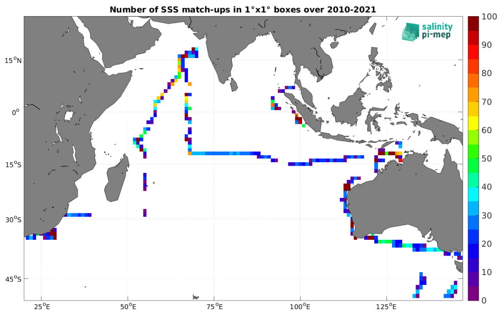
Figure 5: Number of SSS match-ups between TSG (SAMOS) SSS and the CCI SSS L4 Merged-OI v5.5 - 7-day running (ESA) SSS product for the Indian Ocean Pi-MEP region over 1^\circ \times 1^\circ boxes and for the full satellite product period.
