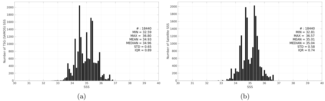
Figure 3: Histograms of SSS from TSG (SAMOS) (a) and CCI SSS L4 Merged-OI v5.5 - 7-day running (ESA) (b) considering all match-up pairs per bins of 0.1 over the Indian Ocean Pi-MEP region and for the full satellite product period.
