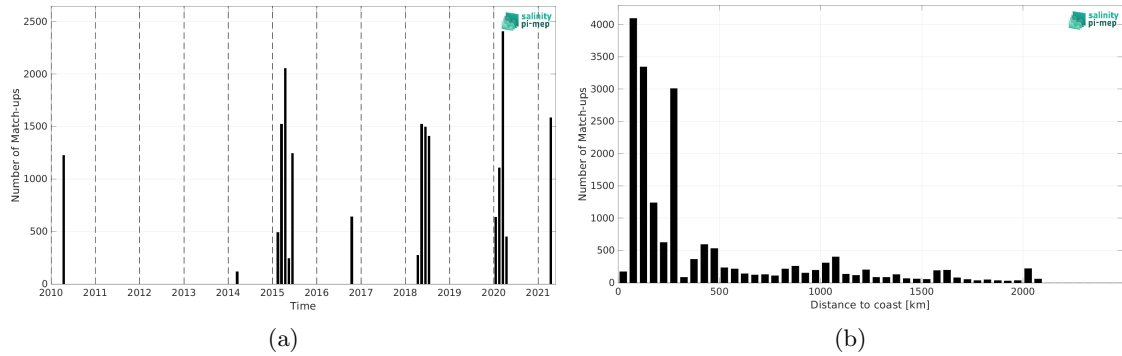
Figure 2: Number of match-ups between TSG (SAMOS) and CCI SSS L4 Merged-OI v5.5 - 7-day running (ESA) SSS as a function of time (a) and as function of the distance to coast (b) over the Indian Ocean Pi-MEP region and for the full satellite product period.
