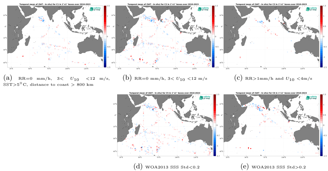
Figure 14: Temporal mean gridded over spatial boxes of size 1^\circ \times 1^\circ of \Delta SSS (CCI SSS L4 Merged-OI v5.5 - 7-day running (ESA) - TSG (LEGOS-DM)) for 5 different subdatasets corresponding to: RR=0 mm/h, 3 < U_{10} < 12 m/s, SST > 5^\circ\text{C} , distance to coast > 800 km (a), RR=0 mm/h, 3 < U_{10} < 12 m/s (b), RR > 1 mm/h and U_{10} < 4 m/s (c), WOA2013 SSS Std < 0.2 (d), WOA2013 SSS Std > 0.2 (e).
