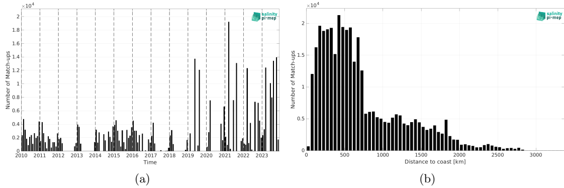
Figure 2: Number of match-ups between TSG (LEGOS-DM) and CCI SSS L4 Merged-OI v5.5 - 7-day running (ESA) SSS as a function of time (a) and as function of the distance to coast (b) over the Indian Ocean Pi-MEP region and for the full satellite product period.
