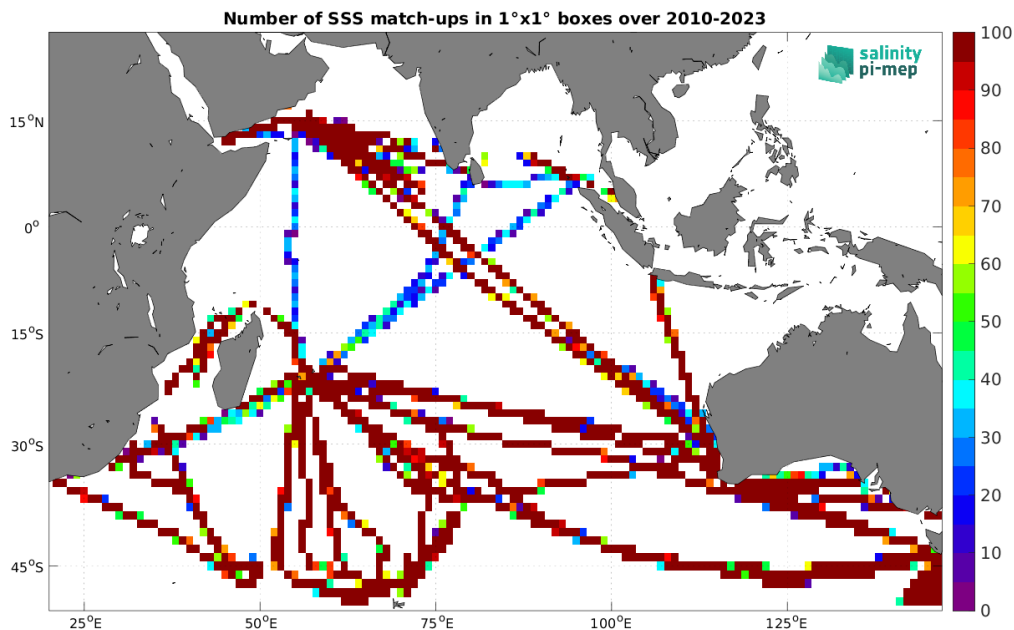
Figure 5: Number of SSS match-ups between TSG (LEGOS-DM) SSS and the CCI SSS L4 Merged-OI v5.5 - 7-day running (ESA) SSS product for the Indian Ocean Pi-MEP region over 1^\circ \times 1^\circ boxes and for the full satellite product period.
