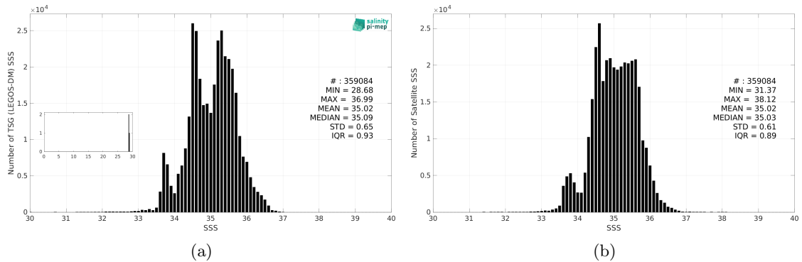
Figure 3: Histograms of SSS from TSG (LEGOS-DM) (a) and CCI SSS L4 Merged-OI v5.5 - 7-day running (ESA) (b) considering all match-up pairs per bins of 0.1 over the Indian Ocean Pi-MEP region and for the full satellite product period.
