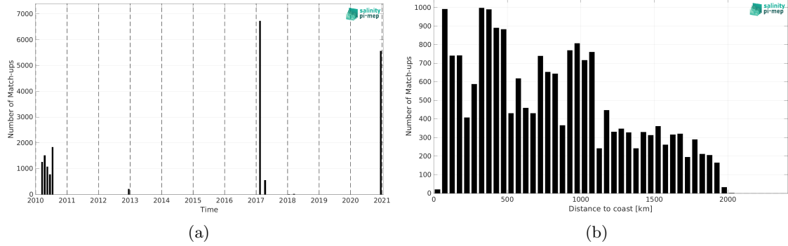
Figure 2: Number of match-ups between TSG (GOSUD-Sailing-ship) and CCI SSS L4 Merged-OI v5.5 - 7-day running (ESA) SSS as a function of time (a) and as function of the distance to coast (b) over the Indian Ocean Pi-MEP region and for the full satellite product period.
