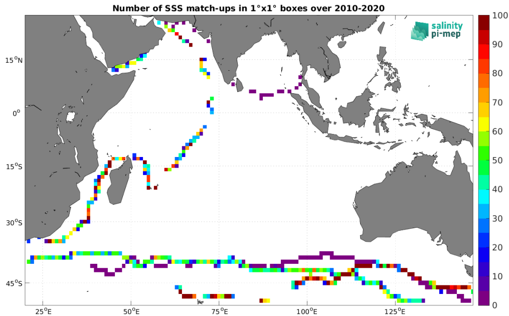
Figure 5: Number of SSS match-ups between TSG (GOSUD-Sailing-ship) SSS and the CCI SSS L4 Merged-OI v5.5 - 7-day running (ESA) SSS product for the Indian Ocean Pi-MEP region over 1^\circ \times 1^\circ boxes and for the full satellite product period.
