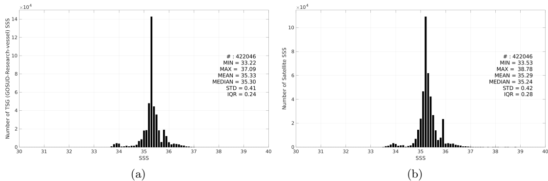
Figure 3: Histograms of SSS from TSG (GOSUD-Research-vessel) (a) and CCI SSS L4 Merged-OI v5.5 - 7-day running (ESA) (b) considering all match-up pairs per bins of 0.1 over the Indian Ocean Pi-MEP region and for the full satellite product period.
