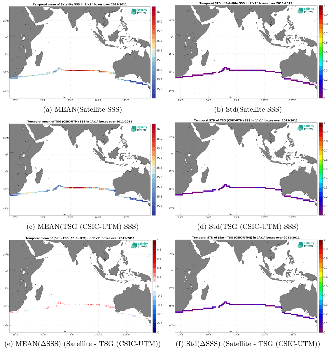
Figure 7: Temporal mean (left) and Std (right) of SSS from CCI SSS L4 Merged-OI v5.5 - 7-day running (ESA) (top), TSG (CSIC-UTM) (middle), and of \Delta SSS (Satellite - TSG (CSIC-UTM)). Only match-up pairs are used to generate these maps.
