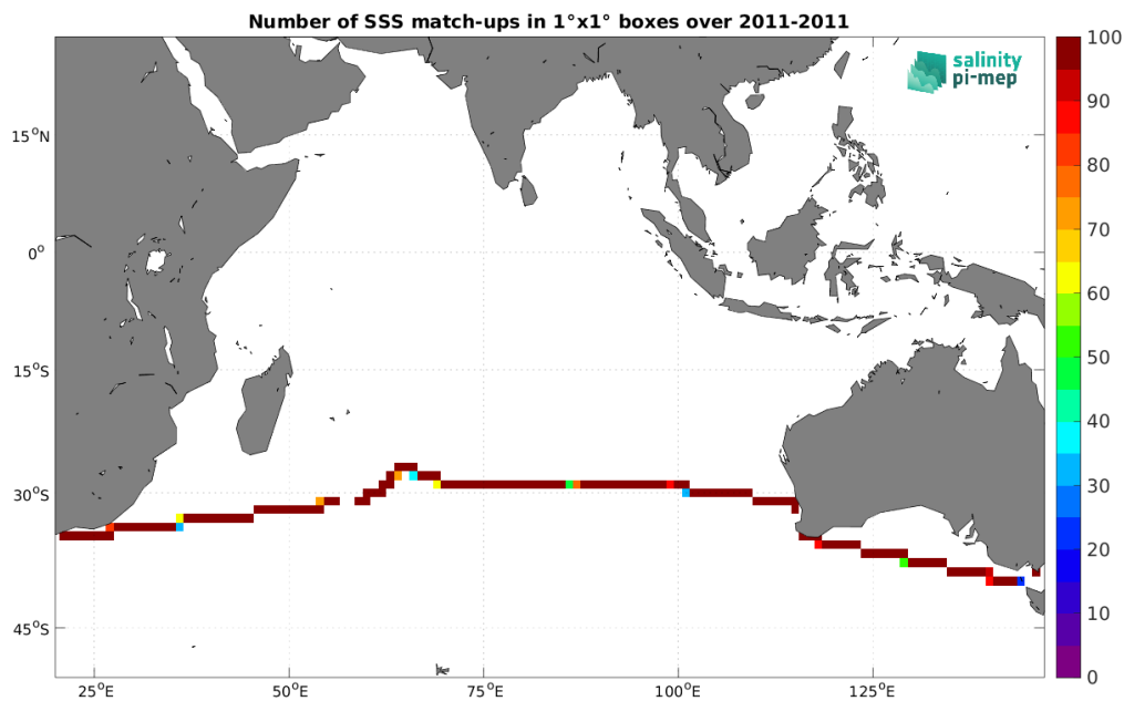
Figure 5: Number of SSS match-ups between TSG (CSIC-UTM) SSS and the CCI SSS L4 Merged-OI v5.5 - 7-day running (ESA) SSS product for the Indian Ocean Pi-MEP region over 1^\circ \times 1^\circ boxes and for the full satellite product period.
