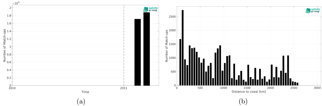
Figure 2: Number of match-ups between TSG (CSIC-UTM) and CCI SSS L4 Merged-OI v5.5 - 7-day running (ESA) SSS as a function of time (a) and as function of the distance to coast (b) over the Indian Ocean Pi-MEP region and for the full satellite product period.
