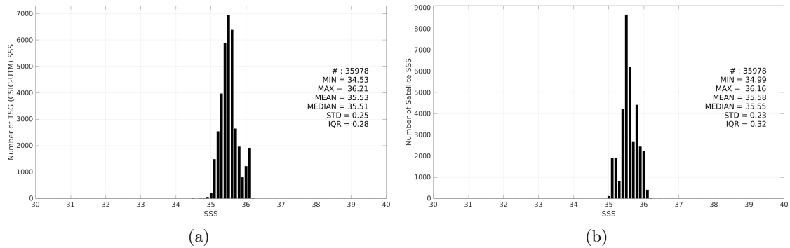
Figure 3: Histograms of SSS from TSG (CSIC-UTM) (a) and CCI SSS L4 Merged-OI v5.5 - 7-day running (ESA) (b) considering all match-up pairs per bins of 0.1 over the Indian Ocean Pi-MEP region and for the full satellite product period.
