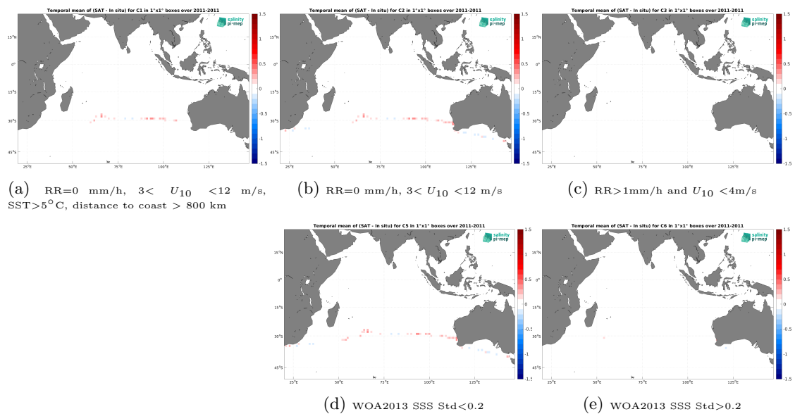
Figure 14: Temporal mean gridded over spatial boxes of size 1^\circ \times 1^\circ of \Delta SSS (CCI SSS L4 Merged-OI v5.5 - 7-day running (ESA) - TSG (CSIC-UTM)) for 5 different subdatasets corresponding to: RR=0 mm/h, 3 < U_{10} < 12 m/s, SST > 5^\circ\text{C} , distance to coast > 800 km (a), RR=0 mm/h, 3 < U_{10} < 12 m/s (b), RR > 1 mm/h and U_{10} < 4 m/s (c), WOA2013 SSS Std < 0.2 (d), WOA2013 SSS Std > 0.2 (e).
