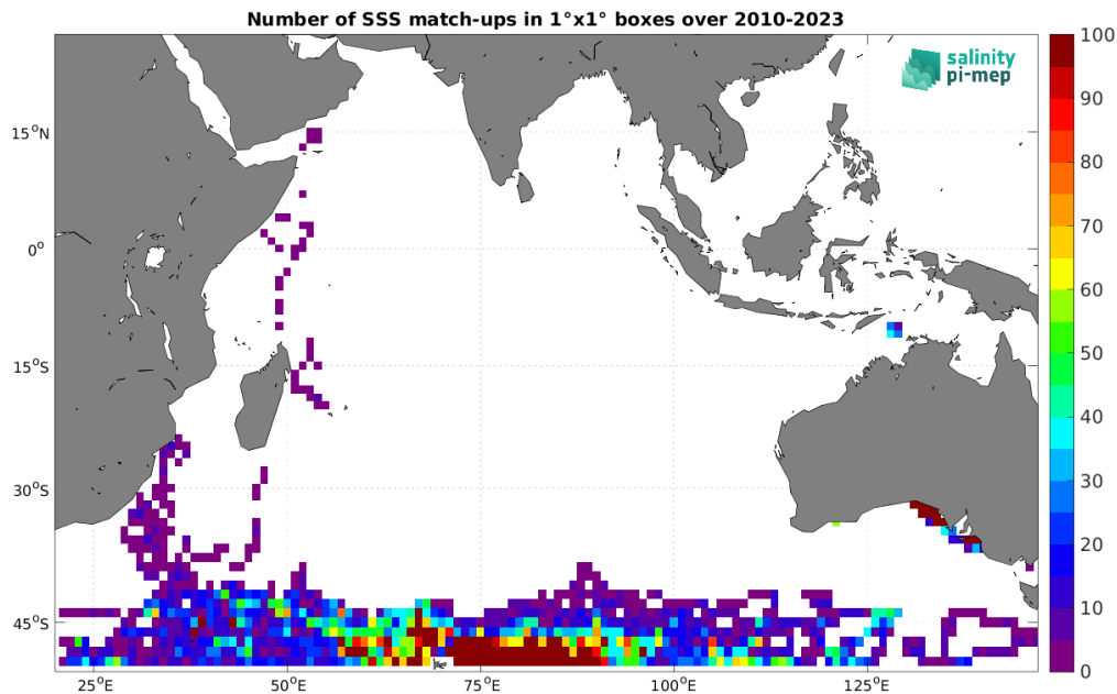
Figure 5: Number of SSS match-ups between Marine mammals SSS and the CCI SSS L4 Merged-OI v5.5 - 7-day running (ESA) SSS product for the Indian Ocean Pi-MEP region over 1^\circ \times 1^\circ boxes and for the full satellite product period.
