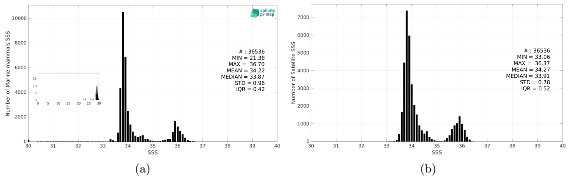
Figure 3: Histograms of SSS from Marine mammals (a) and CCI SSS L4 Merged-OI v5.5 - 7-day running (ESA) (b) considering all match-up pairs per bins of 0.1 over the Indian Ocean Pi-MEP region and for the full satellite product period.
