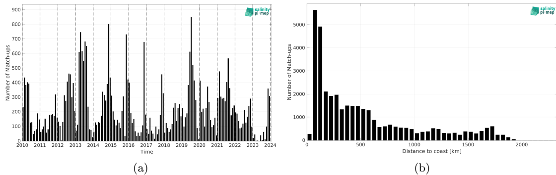
Figure 2: Number of match-ups between Marine mammals and CCI SSS L4 Merged-OI v5.5 - 7-day running (ESA) SSS as a function of time (a) and as function of the distance to coast (b) over the Indian Ocean Pi-MEP region and for the full satellite product period.
