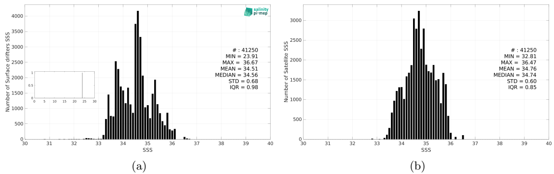
Figure 3: Histograms of SSS from Surface drifters (a) and CCI SSS L4 Merged-OI v5.5 - 7-day running (ESA) (b) considering all match-up pairs per bins of 0.1 over the Indian Ocean Pi-MEP region and for the full satellite product period.
