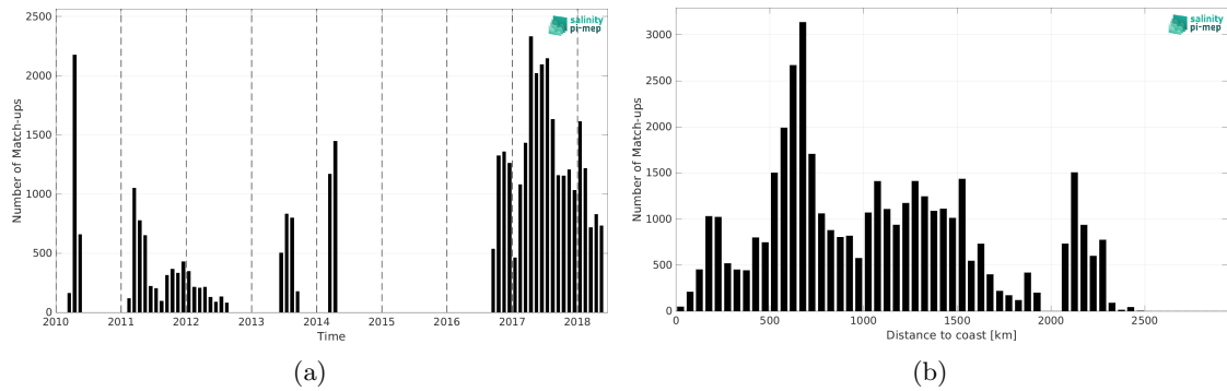
Figure 2: Number of match-ups between Surface drifters and CCI SSS L4 Merged-OI v5.5 - 7-day running (ESA) SSS as a function of time (a) and as function of the distance to coast (b) over the Indian Ocean Pi-MEP region and for the full satellite product period.
