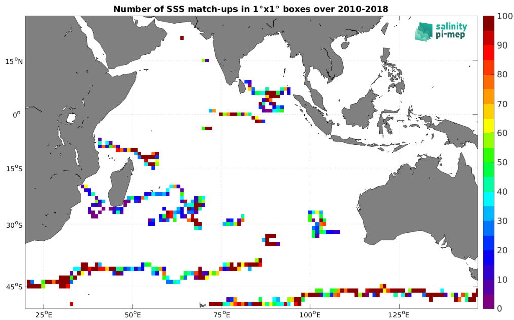
Figure 4: Number of SSS match-ups between Surface drifters SSS and the CCI SSS L4 Merged-OI v5.5 - 7-day running (ESA) SSS product for the Indian Ocean Pi-MEP region over 1^\circ \times 1^\circ boxes and for the full satellite product period.
