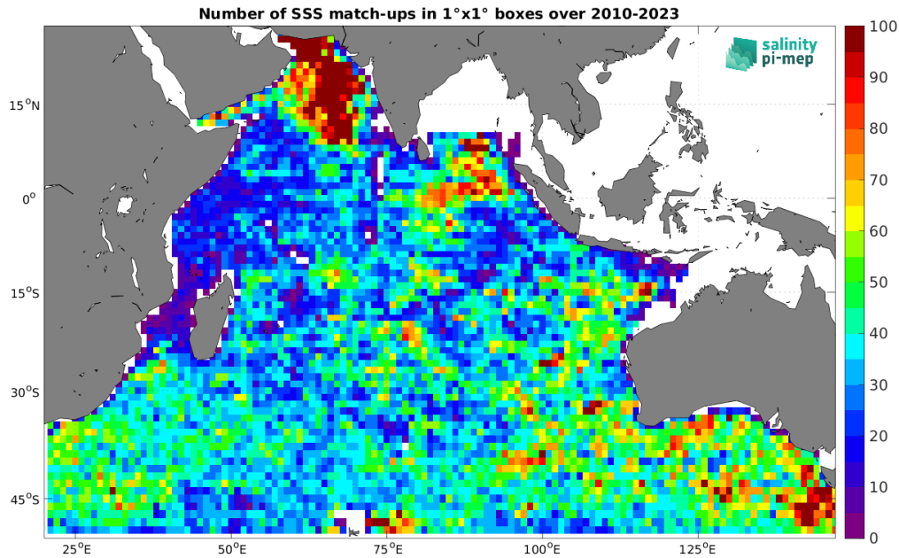
Figure 5: Number of SSS match-ups between Argo SSS and the CCI SSS L4 Merged-OI v5.5 - 7-day running (ESA) SSS product for the Indian Ocean Pi-MEP region over 1^\circ \times 1^\circ boxes and for the full satellite product period.
