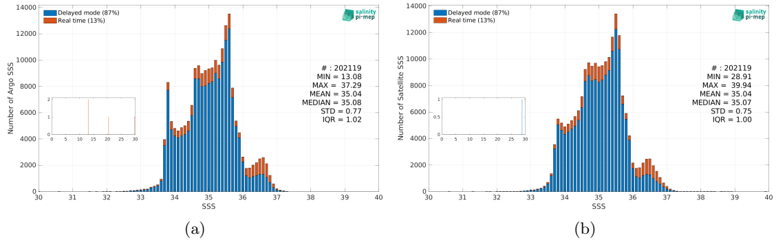
Figure 3: Histograms of SSS from Argo (a) and CCI SSS L4 Merged-OI v5.5 - 7-day running (ESA) (b) considering all match-up pairs per bins of 0.1 over the Indian Ocean Pi-MEP region and for the full satellite product period.
