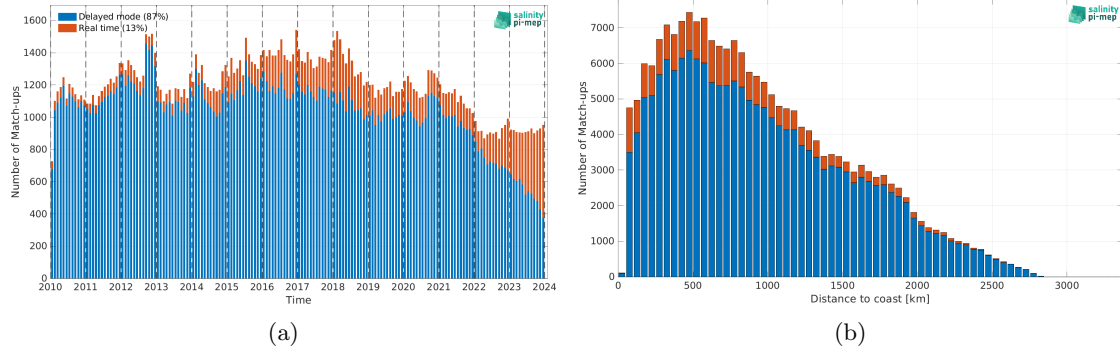
Figure 2: Number of match-ups between Argo and CCI SSS L4 Merged-OI v5.5 - 7-day running (ESA) SSS as a function of time (a) and as function of the distance to coast (b) over the Indian Ocean Pi-MEP region and for the full satellite product period.
