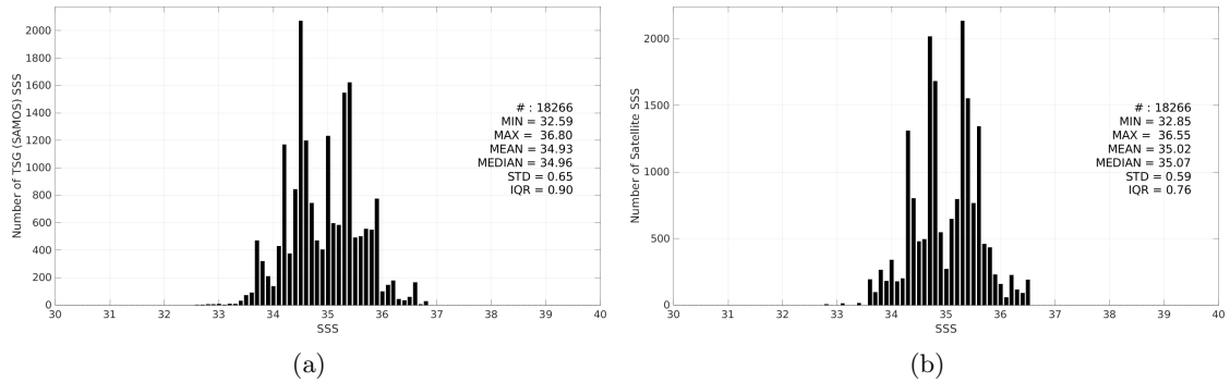
Figure 3: Histograms of SSS from TSG (SAMOS) (a) and CCI SSS L4 Merged-OI v5.5 - 30-day running (ESA) (b) considering all match-up pairs per bins of 0.1 over the Indian Ocean Pi-MEP region and for the full satellite product period.
