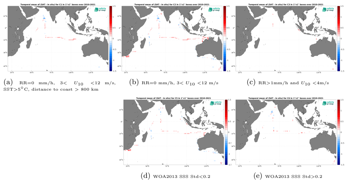
Figure 14: Temporal mean gridded over spatial boxes of size 1^\circ \times 1^\circ of \Delta SSS (CCI SSS L4 Merged-OI v5.5 - 30-day running (ESA) - TSG (SAMOS)) for 5 different subdatasets corresponding to:RR=0 mm/h, 3 < U_{10} < 12 m/s, SST >5^\circ C, distance to coast > 800 km (a), RR=0 mm/h, 3 < U_{10} < 12 m/s (b), RR >1 mm/h and U_{10} < 4 m/s (c), WOA2013 SSS Std <0.2 (d), WOA2013 SSS Std >0.2 (e).
