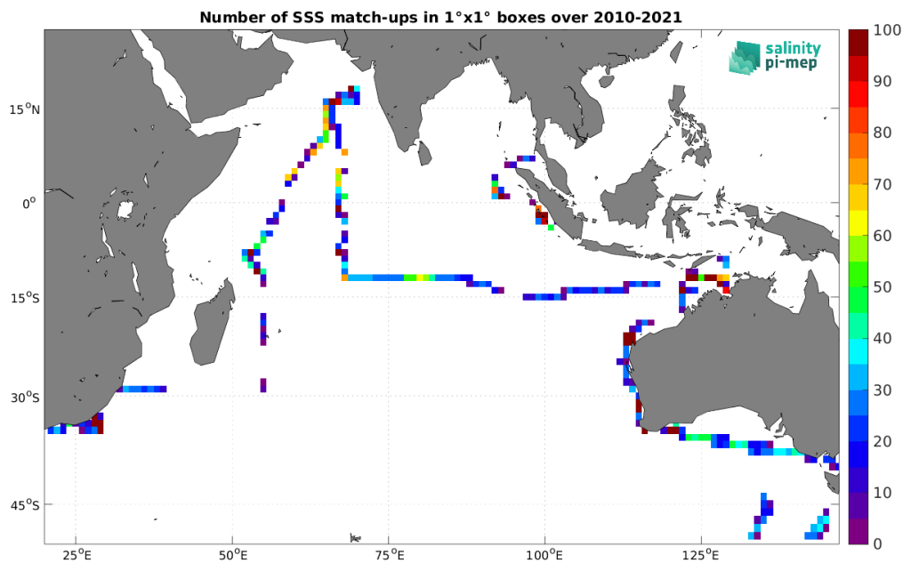
Figure 5: Number of SSS match-ups between TSG (SAMOS) SSS and the CCI SSS L4 Merged-OI v5.5 - 30-day running (ESA) SSS product for the Indian Ocean Pi-MEP region over 1^\circ \times 1^\circ boxes and for the full satellite product period.
