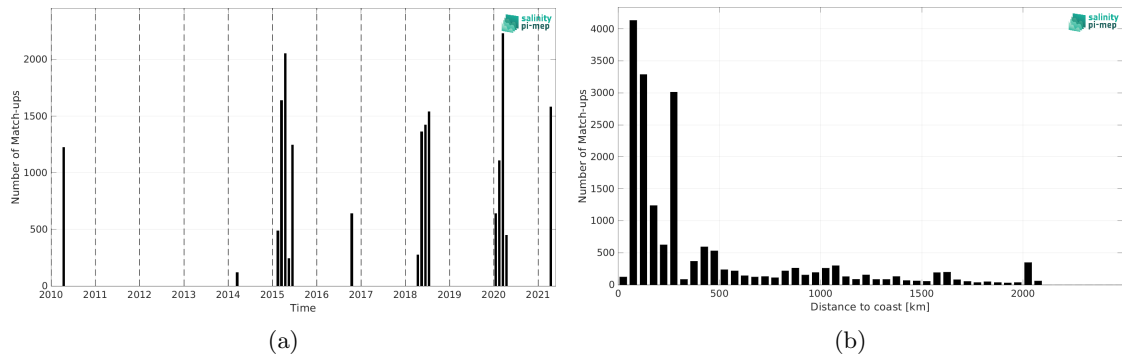
Figure 2: Number of match-ups between TSG (SAMOS) and CCI SSS L4 Merged-OI v5.5 - 30-day running (ESA) SSS as a function of time (a) and as function of the distance to coast (b) over the Indian Ocean Pi-MEP region and for the full satellite product period.
