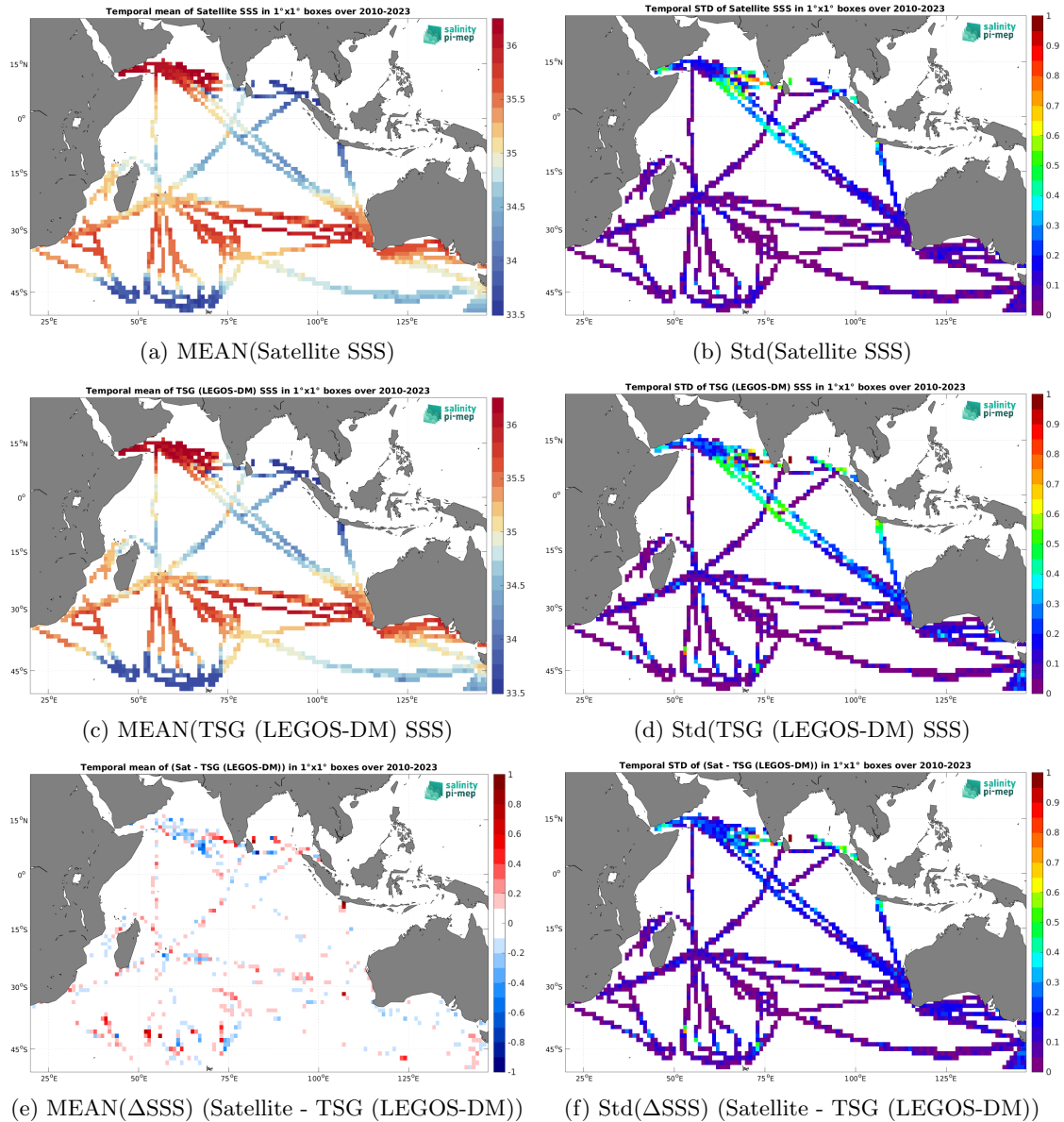
Figure 7: Temporal mean (left) and Std (right) of SSS from CCI SSS L4 Merged-OI v5.5 - 30-day running (ESA) (top), TSG (LEGOS-DM) (middle), and of \Delta SSS (Satellite - TSG (LEGOS-DM)). Only match-up pairs are used to generate these maps.
