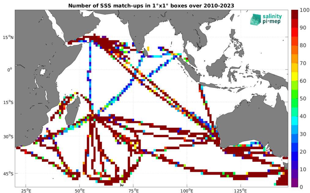
Figure 5: Number of SSS match-ups between TSG (LEGOS-DM) SSS and the CCI SSS L4 Merged-OI v5.5 - 30-day running (ESA) SSS product for the Indian Ocean Pi-MEP region over 1^\circ \times 1^\circ boxes and for the full satellite product period.
