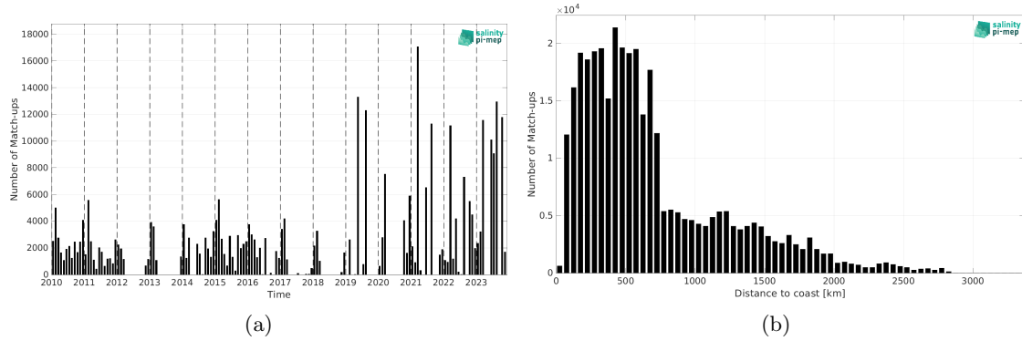
Figure 2: Number of match-ups between TSG (LEGOS-DM) and CCI SSS L4 Merged-OI v5.5 - 30-day running (ESA) SSS as a function of time (a) and as function of the distance to coast (b) over the Indian Ocean Pi-MEP region and for the full satellite product period.
