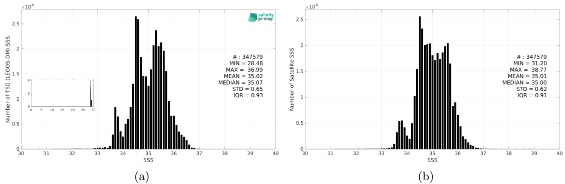
Figure 3: Histograms of SSS from TSG (LEGOS-DM) (a) and CCI SSS L4 Merged-OI v5.5 - 30-day running (ESA) (b) considering all match-up pairs per bins of 0.1 over the Indian Ocean Pi-MEP region and for the full satellite product period.
