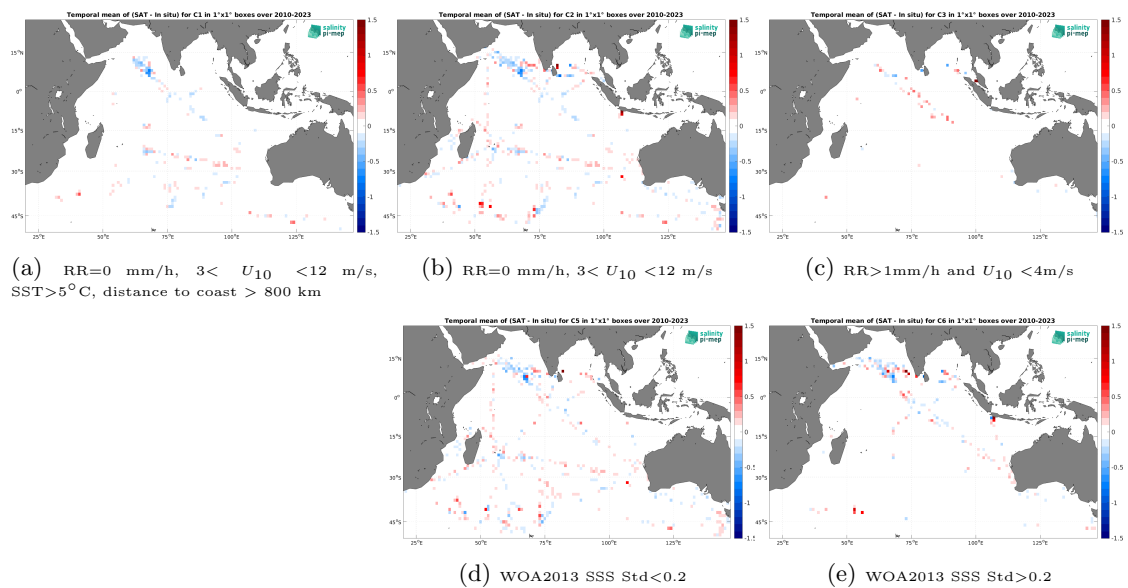
Figure 14: Temporal mean gridded over spatial boxes of size 1^\circ \times 1^\circ of \Delta SSS (CCI SSS L4 Merged-OI v5.5 - 30-day running (ESA) - TSG (LEGOS-DM)) for 5 different subdatasets corresponding to: RR=0 mm/h, 3 < U_{10} < 12 m/s, SST > 5^\circ\text{C} , distance to coast > 800 km (a), RR=0 mm/h, 3 < U_{10} < 12 m/s (b), RR > 1 mm/h and U_{10} < 4 m/s (c), WOA2013 SSS Std < 0.2 (d), WOA2013 SSS Std > 0.2 (e).
