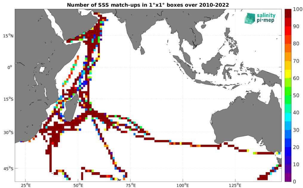
Figure 5: Number of SSS match-ups between TSG (GOSUD-Research-vessel) SSS and the CCI SSS L4 Merged-OI v5.5 - 30-day running (ESA) SSS product for the Indian Ocean Pi-MEP region over 1^\circ \times 1^\circ boxes and for the full satellite product period.
