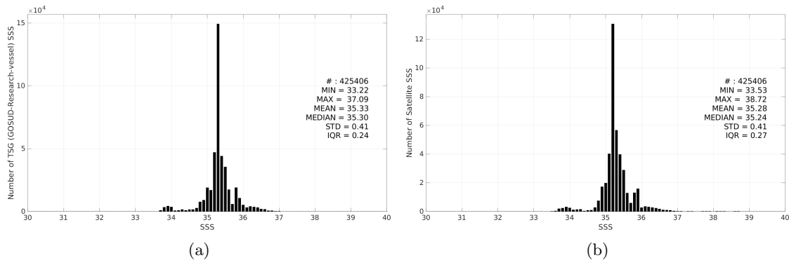
Figure 3: Histograms of SSS from TSG (GOSUD-Research-vessel) (a) and CCI SSS L4 Merged-OI v5.5 - 30-day running (ESA) (b) considering all match-up pairs per bins of 0.1 over the Indian Ocean Pi-MEP region and for the full satellite product period.
