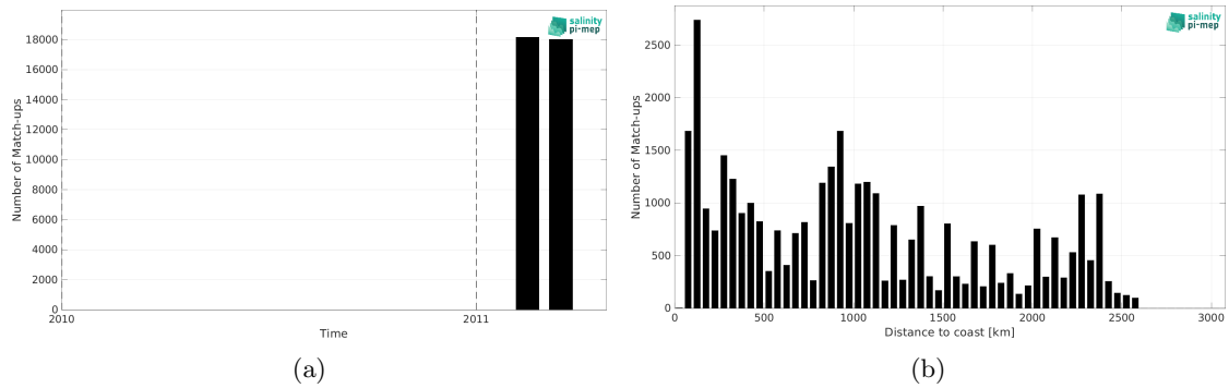
Figure 2: Number of match-ups between TSG (CSIC-UTM) and CCI SSS L4 Merged-OI v5.5 - 30-day running (ESA) SSS as a function of time (a) and as function of the distance to coast (b) over the Indian Ocean Pi-MEP region and for the full satellite product period.
