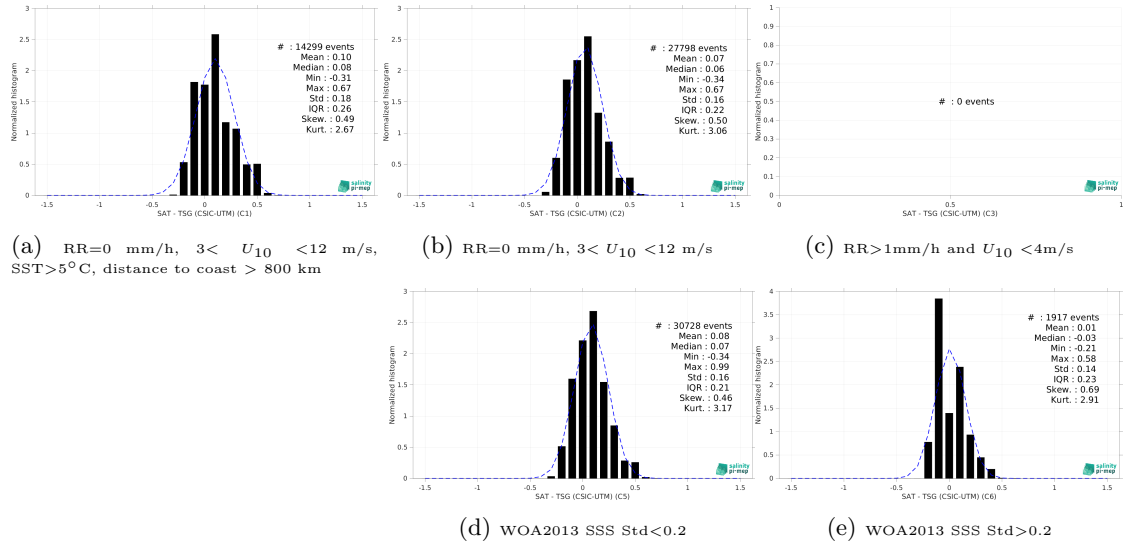
Figure 15: Normalized histogram of \Delta SSS (CCI SSS L4 Merged-OI v5.5 - 30-day running (ESA) - TSG (CSIC-UTM)) for 5 different subdatasets corresponding to: RR=0 mm/h, 3 < U_{10} < 12 m/s, SST > 5°C, distance to coast > 800 km (a), RR=0 mm/h, 3 < U_{10} < 12 m/s (b), RR > 1mm/h and U_{10} < 4 m/s (c), WOA2013 SSS Std < 0.2 (d), WOA2013 SSS Std > 0.2 (e).
