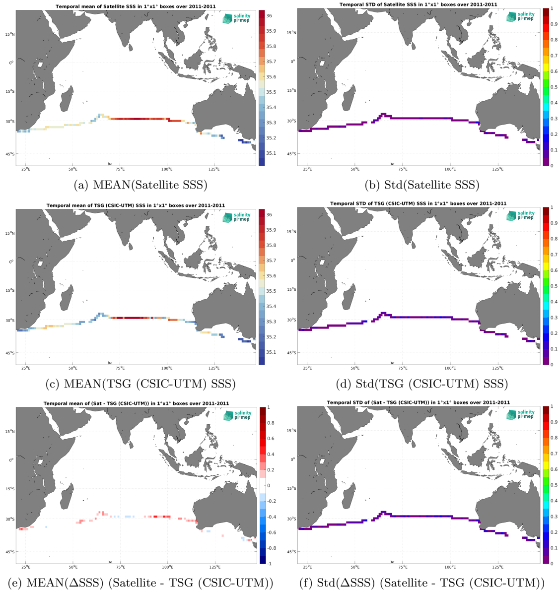
Figure 7: Temporal mean (left) and Std (right) of SSS from CCI SSS L4 Merged-OI v5.5 - 30-day running (ESA) (top), TSG (CSIC-UTM) (middle), and of \Delta SSS (Satellite - TSG (CSIC-UTM)). Only match-up pairs are used to generate these maps.
