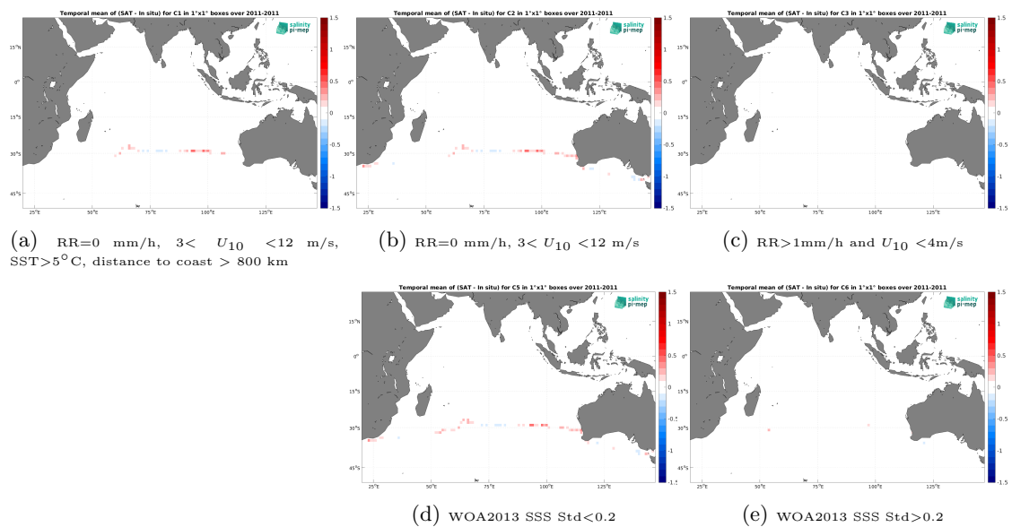
Figure 14: Temporal mean gridded over spatial boxes of size 1^\circ \times 1^\circ of \Delta SSS (CCI SSS L4 Merged-OI v5.5 - 30-day running (ESA) - TSG (CSIC-UTM)) for 5 different subdatasets corresponding to:RR=0 mm/h, 3 < U_{10} < 12 m/s, SST >5^\circ\text{C} , distance to coast > 800 km (a), RR=0 mm/h, 3 < U_{10} < 12 m/s (b), RR >1 mm/h and U_{10} < 4 m/s (c), WOA2013 SSS Std <0.2 (d), WOA2013 SSS Std >0.2 (e).
