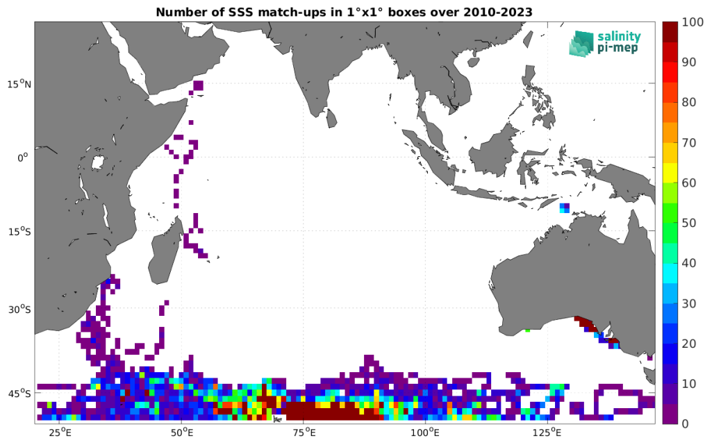
Figure 5: Number of SSS match-ups between Marine mammals SSS and the CCI SSS L4 Merged-OI v5.5 - 30-day running (ESA) SSS product for the Indian Ocean Pi-MEP region over 1^\circ \times 1^\circ boxes and for the full satellite product period.
