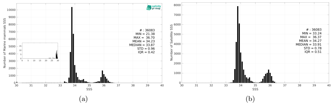
Figure 3: Histograms of SSS from Marine mammals (a) and CCI SSS L4 Merged-OI v5.5 - 30-day running (ESA) (b) considering all match-up pairs per bins of 0.1 over the Indian Ocean Pi-MEP region and for the full satellite product period.
