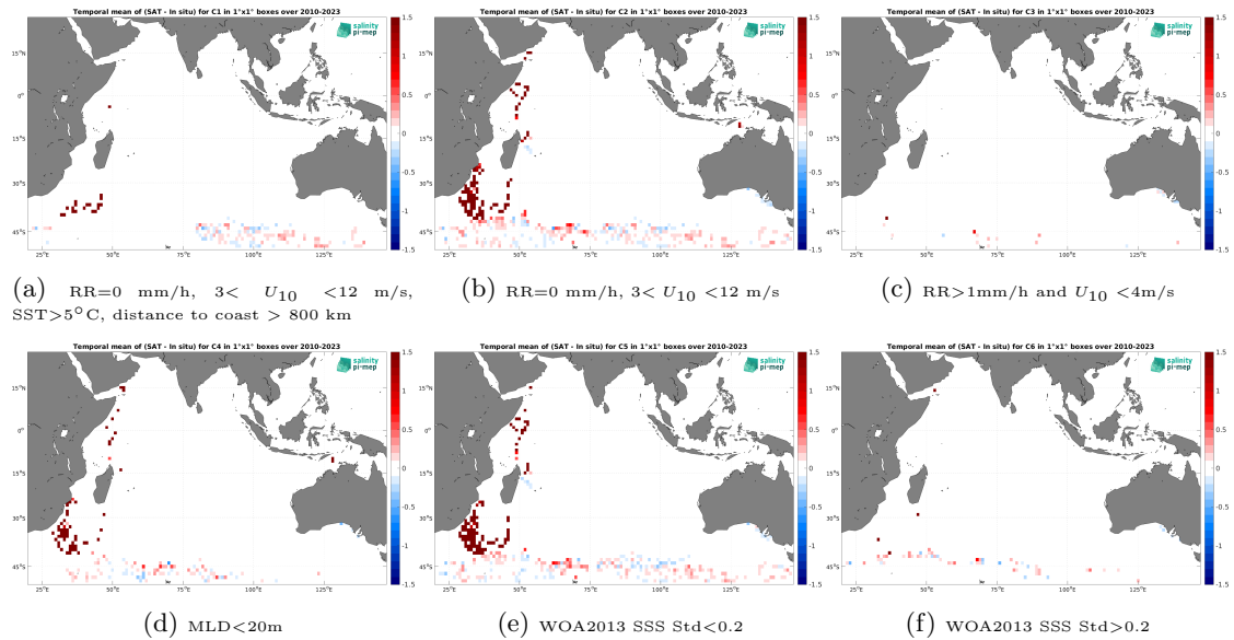
Figure 14: Temporal mean gridded over spatial boxes of size 1^\circ \times 1^\circ of \Delta\text{SSS} (CCI SSS L4 Merged-OI v5.5 - 30-day running (ESA) - Marine mammals) for 6 different subdatasets corresponding to:RR=0 mm/h, 3 < U_{10} < 12 m/s, SST>5°C, distance to coast > 800 km (a), RR=0 mm/h, 3 < U_{10} < 12 m/s (b), RR>1mm/h and U_{10} < 4 m/s (c),MLD<20m (d),WOA2013 SSS Std<0.2 (e),WOA2013 SSS Std>0.2 (f).
