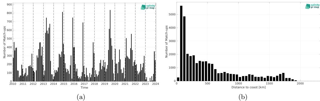
Figure 2: Number of match-ups between Marine mammals and CCI SSS L4 Merged-OI v5.5 - 30-day running (ESA) SSS as a function of time (a) and as function of the distance to coast (b) over the Indian Ocean Pi-MEP region and for the full satellite product period.
