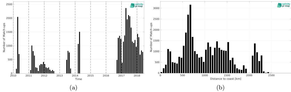
Figure 2: Number of match-ups between Surface drifters and CCI SSS L4 Merged-OI v5.5 - 30-day running (ESA) SSS as a function of time (a) and as function of the distance to coast (b) over the Indian Ocean Pi-MEP region and for the full satellite product period.
