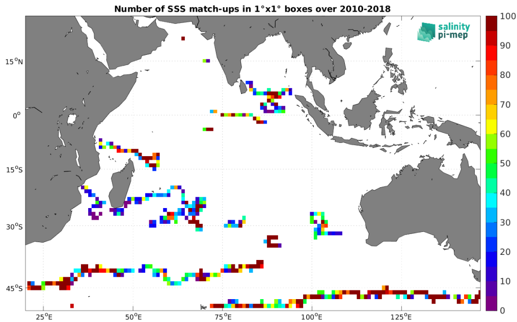
Figure 4: Number of SSS match-ups between Surface drifters SSS and the CCI SSS L4 Merged-OI v5.5 - 30-day running (ESA) SSS product for the Indian Ocean Pi-MEP region over 1°x1° boxes and for the full satellite product period.
