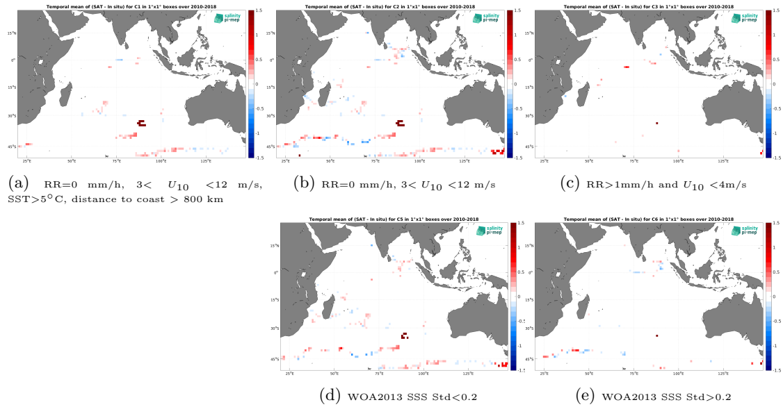
Figure 13: Temporal mean gridded over spatial boxes of size 1^\circ \times 1^\circ of \Delta SSS (CCI SSS L4 Merged-OI v5.5 - 30-day running (ESA) - Surface drifters) for 5 different subdatasets corresponding to: RR=0 mm/h, 3 < U_{10} < 12 m/s, SST > 5^\circ\text{C} , distance to coast > 800 km (a), RR=0 mm/h, 3 < U_{10} < 12 m/s (b), RR > 1\text{mm/h} and U_{10} < 4\text{m/s} (c), WOA2013 SSS Std < 0.2 (d), WOA2013 SSS Std > 0.2 (e).
