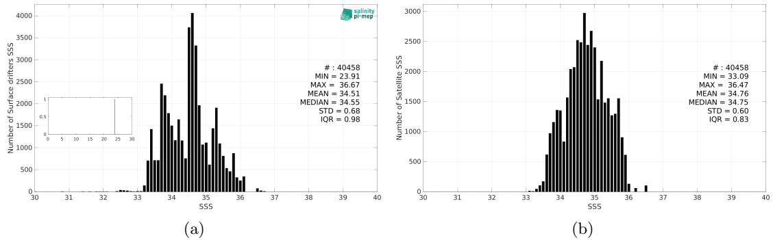
Figure 3: Histograms of SSS from Surface drifters (a) and CCI SSS L4 Merged-OI v5.5 - 30-day running (ESA) (b) considering all match-up pairs per bins of 0.1 over the Indian Ocean Pi-MEP region and for the full satellite product period.
