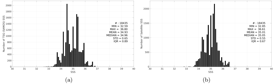
Figure 3: Histograms of SSS from TSG (SAMOS) (a) and CCI SSS L4 Merged-OI v4.41 - 7-day running (ESA) (b) considering all match-up pairs per bins of 0.1 over the Indian Ocean Pi-MEP region and for the full satellite product period.
