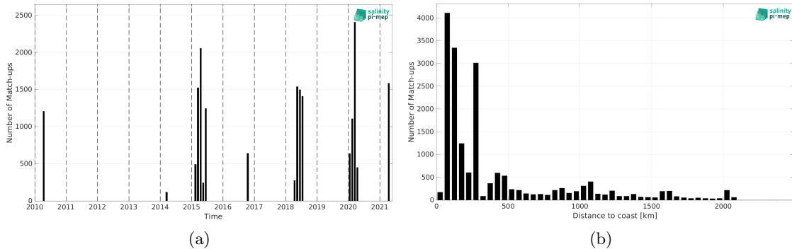
Figure 2: Number of match-ups between TSG (SAMOS) and CCI SSS L4 Merged-OI v4.41 - 7-day running (ESA) SSS as a function of time (a) and as function of the distance to coast (b) over the Indian Ocean Pi-MEP region and for the full satellite product period.
