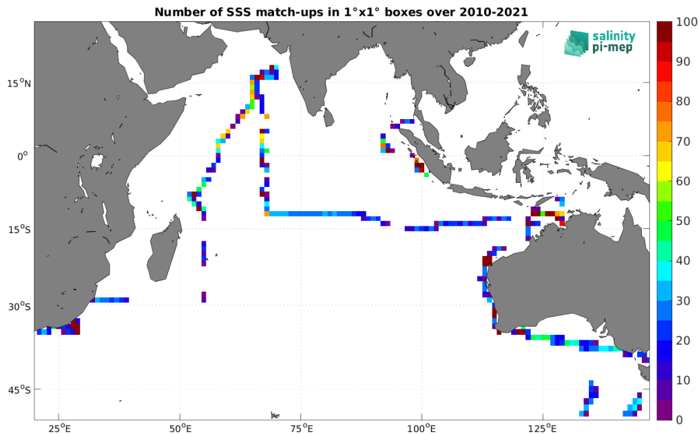
Figure 5: Number of SSS match-ups between TSG (SAMOS) SSS and the CCI SSS L4 Merged-OI v4.41 - 7-day running (ESA) SSS product for the Indian Ocean Pi-MEP region over 1^\circ \times 1^\circ boxes and for the full satellite product period.
