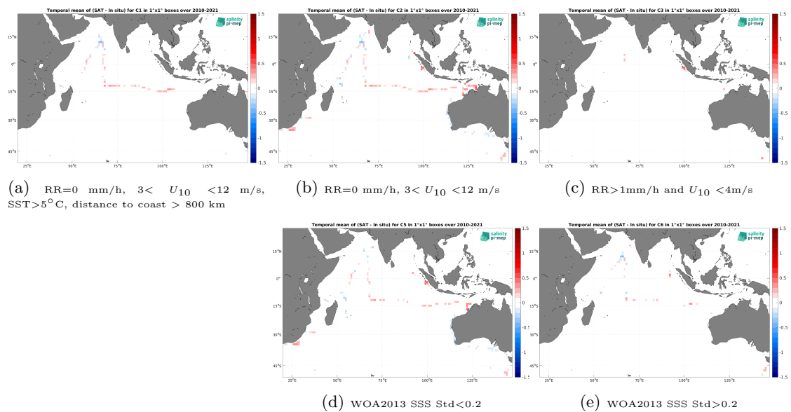
Figure 14: Temporal mean gridded over spatial boxes of size 1^\circ \times 1^\circ of \Delta SSS (CCI SSS L4 Merged-OI v4.41 - 7-day running (ESA) - TSG (SAMOS)) for 5 different subdatasets corresponding to: RR=0 mm/h, 3 < U_{10} < 12 m/s, SST > 5^\circ\text{C} , distance to coast > 800 km (a), RR=0 mm/h, 3 < U_{10} < 12 m/s (b), RR > 1 mm/h and U_{10} < 4 m/s (c), WOA2013 SSS Std < 0.2 (d), WOA2013 SSS Std > 0.2 (e).
