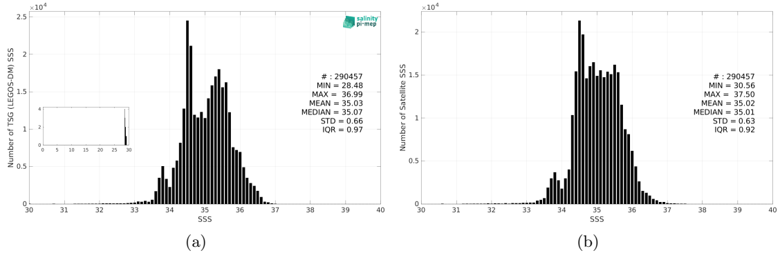
Figure 3: Histograms of SSS from TSG (LEGOS-DM) (a) and CCI SSS L4 Merged-OI v4.41 - 7-day running (ESA) (b) considering all match-up pairs per bins of 0.1 over the Indian Ocean Pi-MEP region and for the full satellite product period.
