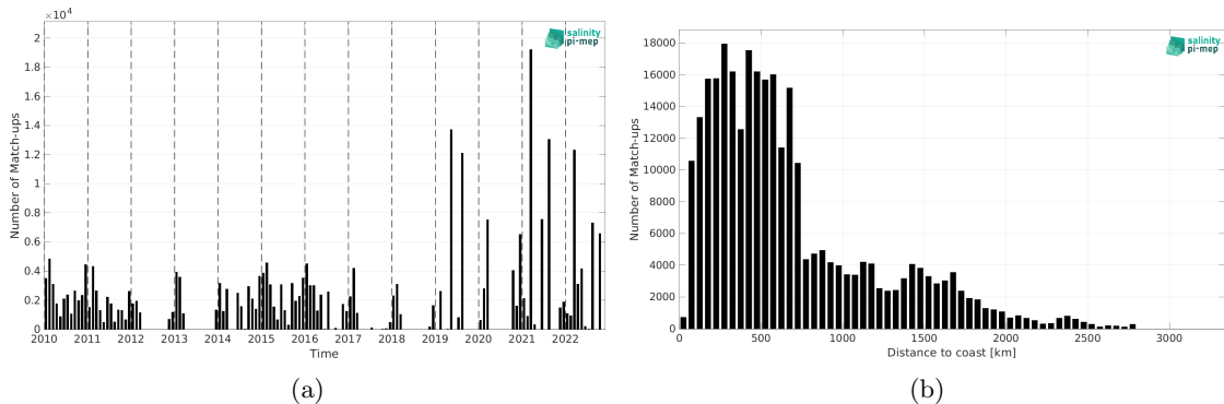
Figure 2: Number of match-ups between TSG (LEGOS-DM) and CCI SSS L4 Merged-OI v4.41 - 7-day running (ESA) SSS as a function of time (a) and as function of the distance to coast (b) over the Indian Ocean Pi-MEP region and for the full satellite product period.
