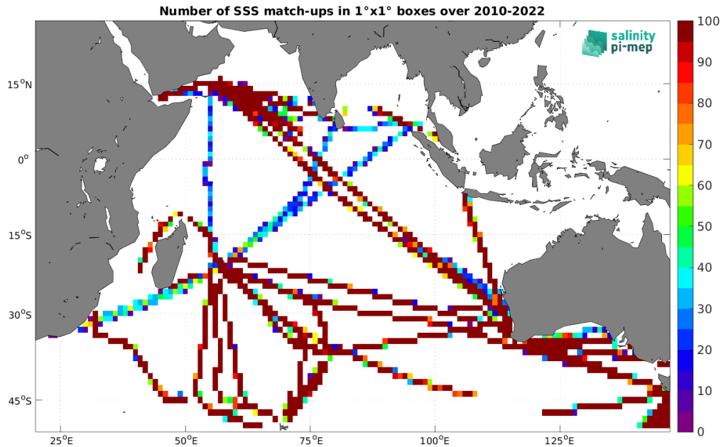
Figure 5: Number of SSS match-ups between TSG (LEGOS-DM) SSS and the CCI SSS L4 Merged-OI v4.41 - 7-day running (ESA) SSS product for the Indian Ocean Pi-MEP region over 1^\circ \times 1^\circ boxes and for the full satellite product period.
