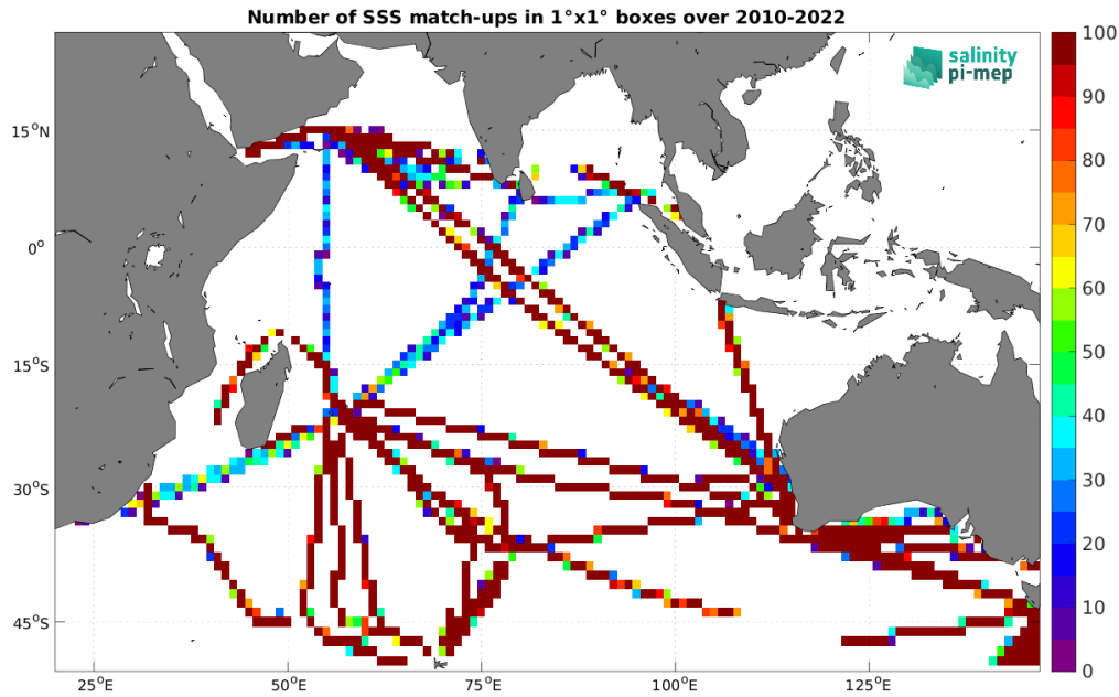
Figure 5: Number of SSS match-ups between TSG (LEGOS-DM) SSS and the CCI SSS L4 Merged-OI v4.41 - 7-day running (ESA) SSS product for the Indian Ocean Pi-MEP region over 1^\circ \times 1^\circ boxes and for the full satellite product period.
