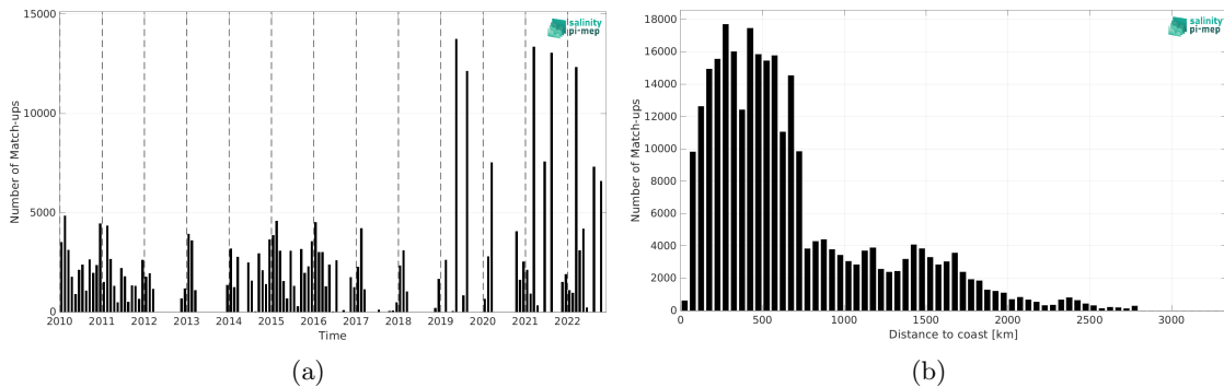
Figure 2: Number of match-ups between TSG (LEGOS-DM) and CCI SSS L4 Merged-OI v4.41 - 7-day running (ESA) SSS as a function of time (a) and as function of the distance to coast (b) over the Indian Ocean Pi-MEP region and for the full satellite product period.
