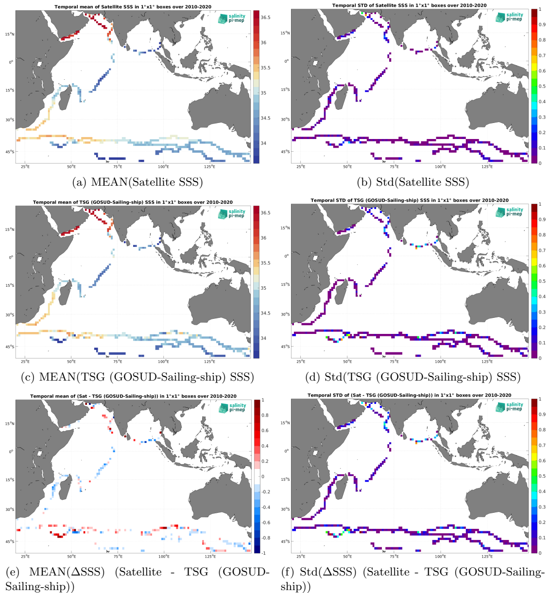
Figure 7: Temporal mean (left) and Std (right) of SSS from CCI SSS L4 Merged-OI v4.41 - 7-day running (ESA) (top), TSG (GOSUD-Sailing-ship) (middle), and of \Delta SSS (Satellite - TSG (GOSUD-Sailing-ship)). Only match-up pairs are used to generate these maps.
