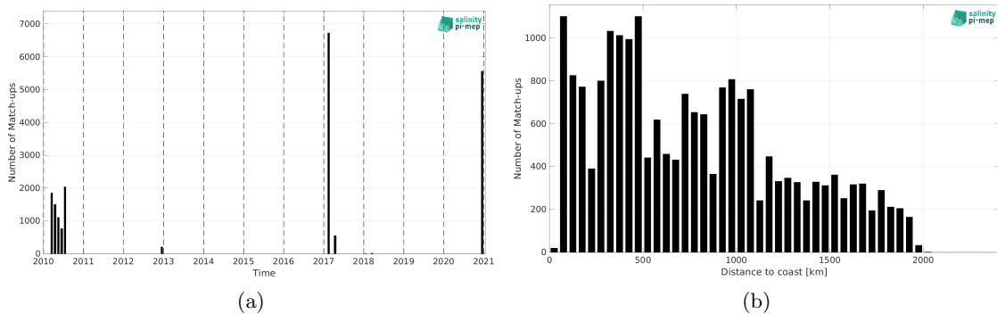
Figure 2: Number of match-ups between TSG (GOSUD-Sailing-ship) and CCI SSS L4 Merged-OI v4.41 - 7-day running (ESA) SSS as a function of time (a) and as function of the distance to coast (b) over the Indian Ocean Pi-MEP region and for the full satellite product period.
