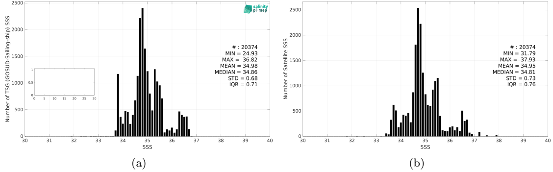
Figure 3: Histograms of SSS from TSG (GOSUD-Sailing-ship) (a) and CCI SSS L4 Merged-OI v4.41 - 7-day running (ESA) (b) considering all match-up pairs per bins of 0.1 over the Indian Ocean Pi-MEP region and for the full satellite product period.
