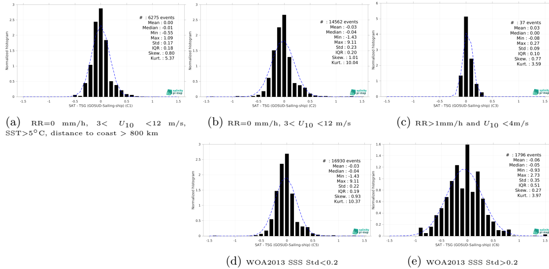
Figure 15: Normalized histogram of \Delta\text{SSS} (CCI SSS L4 Merged-OI v4.41 - 7-day running (ESA) - TSG (GOSUD-Sailing-ship)) for 5 different subdatasets corresponding to: RR=0 mm/h, 3 < U_{10} < 12 m/s, SST>5°C, distance to coast > 800 km (a), RR=0 mm/h, 3 < U_{10} < 12 m/s (b), RR>1mm/h and U_{10} < 4 m/s (c), WOA2013 SSS Std<0.2 (d), WOA2013 SSS Std>0.2 (e).
