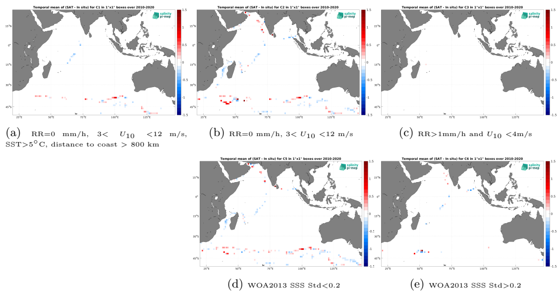
Figure 14: Temporal mean gridded over spatial boxes of size 1^\circ \times 1^\circ of \Delta\text{SSS} (CCI SSS L4 Merged-OI v4.41 - 7-day running (ESA) - TSG (GOSUD-Sailing-ship)) for 5 different subdatasets corresponding to:RR=0 mm/h, 3 < U_{10} < 12 m/s, SST >5^\circ\text{C} , distance to coast > 800 km (a), RR=0 mm/h, 3 < U_{10} < 12 m/s (b), RR >1 mm/h and U_{10} < 4 m/s (c), WOA2013 SSS Std <0.2 (d), WOA2013 SSS Std >0.2 (e).
