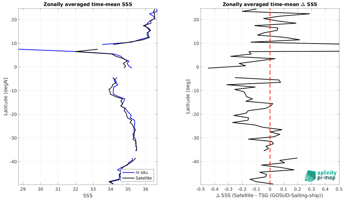
Figure 9: Left panel: Zonal mean SSS from CCI SSS L4 Merged-OI v4.41 - 7-day running (ESA) satellite product (black) and from TSG (GOSUD-Sailing-ship) (blue). Right panel: Zonal mean of \Delta SSS (Satellite - TSG (GOSUD-Sailing-ship)) for all the collected Pi-MEP match-up pairs estimated over the full satellite product period.
