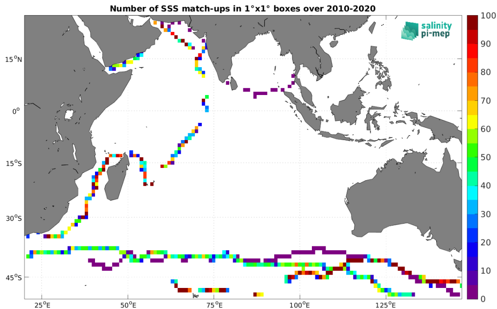
Figure 5: Number of SSS match-ups between TSG (GOSUD-Sailing-ship) SSS and the CCI SSS L4 Merged-OI v4.41 - 7-day running (ESA) SSS product for the Indian Ocean Pi-MEP region over 1^\circ \times 1^\circ boxes and for the full satellite product period.
