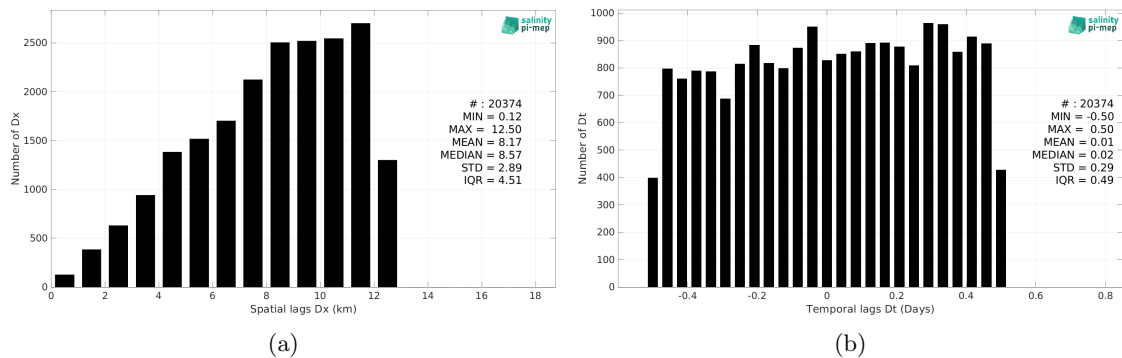
Figure 6: Histograms of the spatial (a) and temporal (b) lags between the location/time of the TSG (GOSUD-Sailing-ship) measurement and the date of the corresponding CCI SSS L4 Merged-OI v4.41 - 7-day running (ESA) SSS pixel.
