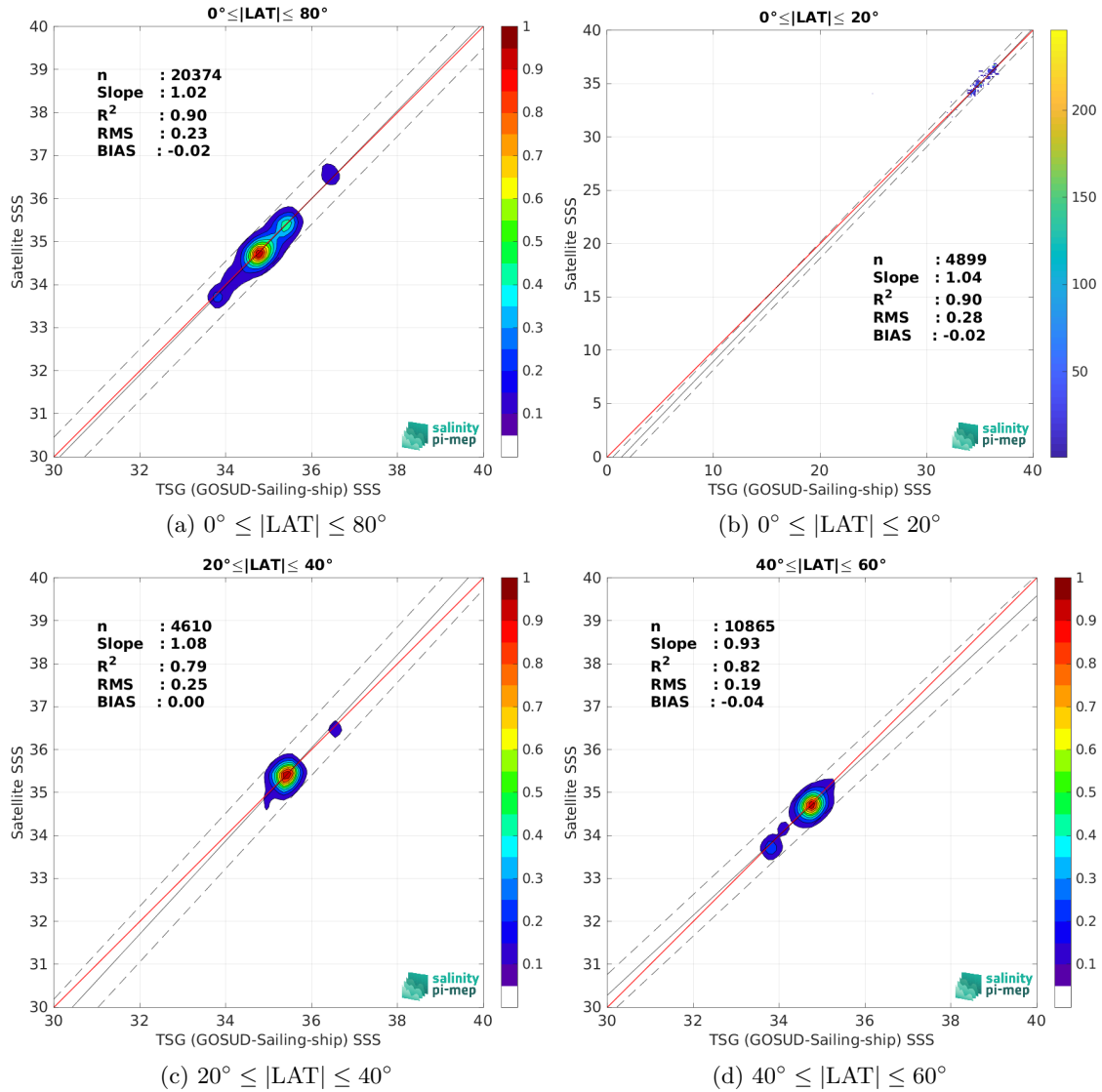
Figure 10: Contour maps of the concentration of CCI SSS L4 Merged-OI v4.41 - 7-day running (ESA) SSS (y-axis) versus TSG (GOSUD-Sailing-ship) SSS (x-axis) at match-up pairs for different latitude bands. For each plot, the red line shows x=y . The black thin and dashed lines indicate a linear fit through the data cloud and the \pm 95\% confidence levels, respectively. The number match-up pairs n , the slope and R^2 coefficient of the linear fit, the root mean square (RMS) and the mean bias between satellite and in situ data are indicated for each latitude band in each plots.
