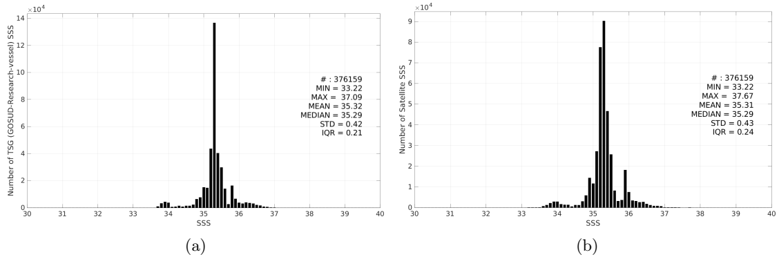
Figure 3: Histograms of SSS from TSG (GOSUD-Research-vessel) (a) and CCI SSS L4 Merged-OI v4.41 - 7-day running (ESA) (b) considering all match-up pairs per bins of 0.1 over the Indian Ocean Pi-MEP region and for the full satellite product period.
