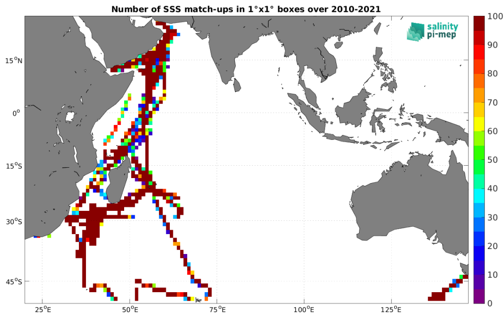
Figure 5: Number of SSS match-ups between TSG (GOSUD-Research-vessel) SSS and the CCI SSS L4 Merged-OI v4.41 - 7-day running (ESA) SSS product for the Indian Ocean Pi-MEP region over 1^\circ \times 1^\circ boxes and for the full satellite product period.
