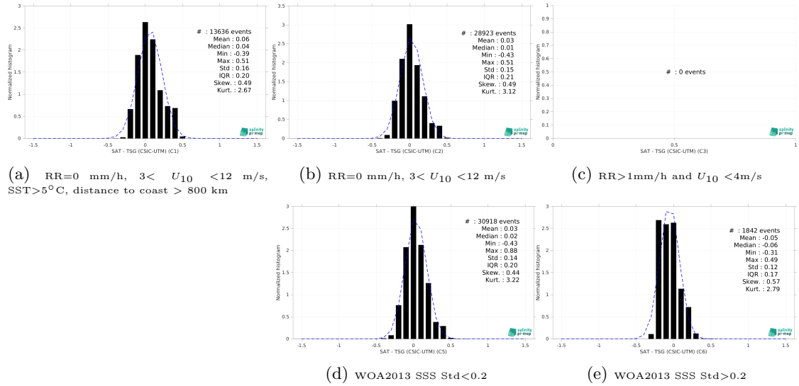
Figure 15: Normalized histogram of \Delta SSS (CCI SSS L4 Merged-OI v4.41 - 7-day running (ESA) - TSG (CSIC-UTM)) for 5 different subdatasets corresponding to: RR=0 mm/h, 3 < U_{10} < 12 m/s, SST > 5°C, distance to coast > 800 km (a), RR=0 mm/h, 3 < U_{10} < 12 m/s (b), RR > 1mm/h and U_{10} < 4 m/s (c), WOA2013 SSS Std < 0.2 (d), WOA2013 SSS Std > 0.2 (e).
