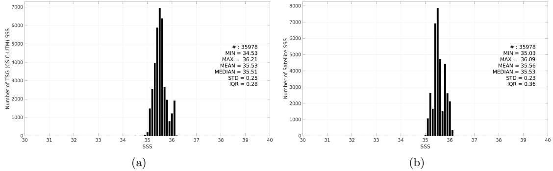
Figure 3: Histograms of SSS from TSG (CSIC-UTM) (a) and CCI SSS L4 Merged-OI v4.41 - 7-day running (ESA) (b) considering all match-up pairs per bins of 0.1 over the Indian Ocean Pi-MEP region and for the full satellite product period.
