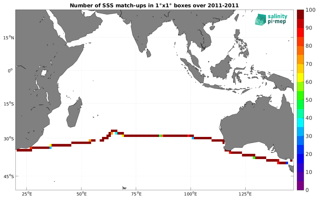
Figure 5: Number of SSS match-ups between TSG (CSIC-UTM) SSS and the CCI SSS L4 Merged-OI v4.41 - 7-day running (ESA) SSS product for the Indian Ocean Pi-MEP region over 1^\circ \times 1^\circ boxes and for the full satellite product period.
