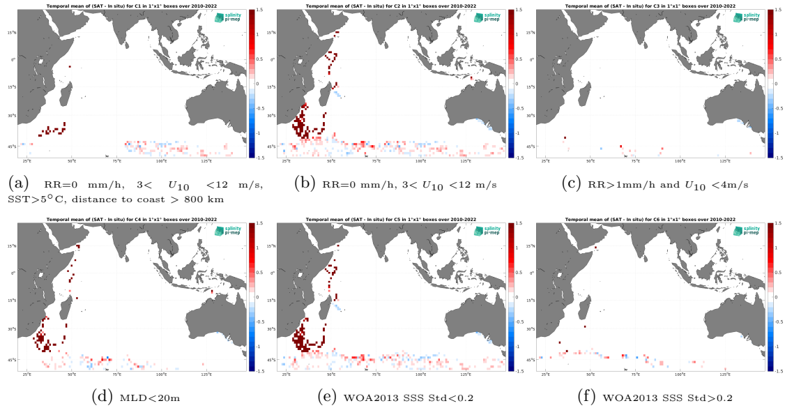
Figure 14: Temporal mean gridded over spatial boxes of size 1^\circ \times 1^\circ of \Delta\text{SSS} (CCI SSS L4 Merged-OI v4.41 - 7-day running (ESA) - Marine mammals) for 6 different subdatasets corresponding to:RR=0 mm/h, 3 < U_{10} < 12 m/s, SST>5°C, distance to coast > 800 km (a), RR=0 mm/h, 3 < U_{10} < 12 m/s (b), RR>1mm/h and U_{10} < 4 m/s (c),MLD<20m (d),WOA2013 SSS Std<0.2 (e),WOA2013 SSS Std>0.2 (f).
