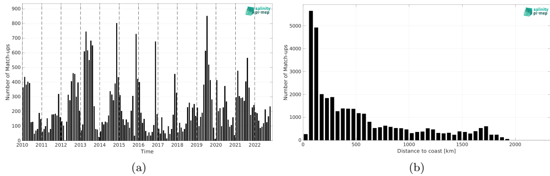
Figure 2: Number of match-ups between Marine mammals and CCI SSS L4 Merged-OI v4.41 - 7-day running (ESA) SSS as a function of time (a) and as function of the distance to coast (b) over the Indian Ocean Pi-MEP region and for the full satellite product period.
