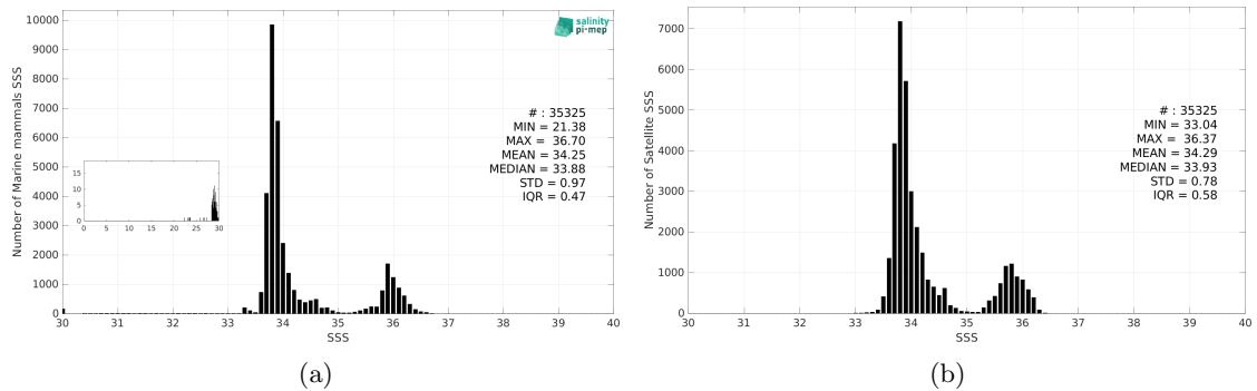
Figure 3: Histograms of SSS from Marine mammals (a) and CCI SSS L4 Merged-OI v4.41 - 7-day running (ESA) (b) considering all match-up pairs per bins of 0.1 over the Indian Ocean Pi-MEP region and for the full satellite product period.
