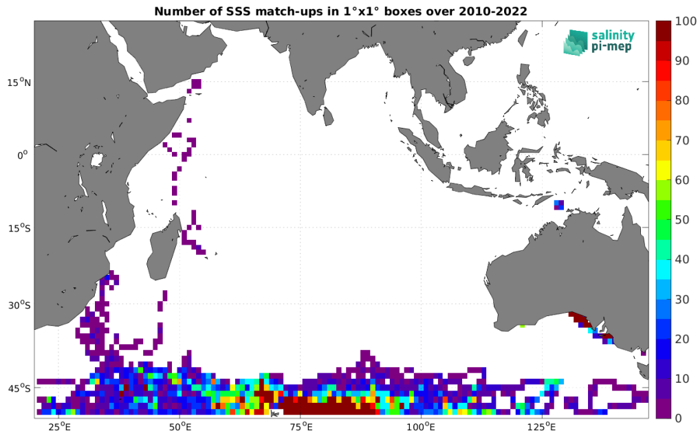
Figure 5: Number of SSS match-ups between Marine mammals SSS and the CCI SSS L4 Merged-OI v4.41 - 7-day running (ESA) SSS product for the Indian Ocean Pi-MEP region over 1^\circ \times 1^\circ boxes and for the full satellite product period.
