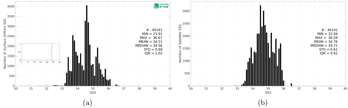
Figure 3: Histograms of SSS from Surface drifters (a) and CCI SSS L4 Merged-OI v4.41 - 7-day running (ESA) (b) considering all match-up pairs per bins of 0.1 over the Indian Ocean Pi-MEP region and for the full satellite product period.
