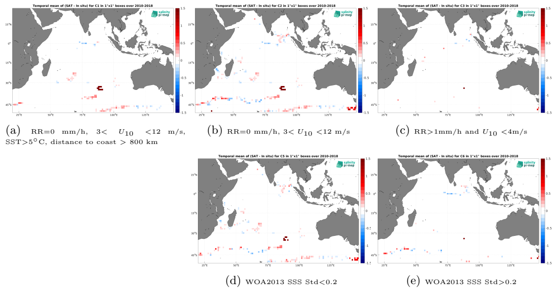
Figure 13: Temporal mean gridded over spatial boxes of size 1^\circ \times 1^\circ of \Delta SSS (CCI SSS L4 Merged-OI v4.41 - 7-day running (ESA) - Surface drifters) for 5 different subdatasets corresponding to:RR=0 mm/h, 3 < U_{10} < 12 m/s, SST >5^\circ C, distance to coast > 800 km (a), RR=0 mm/h, 3 < U_{10} < 12 m/s (b), RR >1 mm/h and U_{10} < 4 m/s (c), WOA2013 SSS Std <0.2 (d), WOA2013 SSS Std >0.2 (e).
