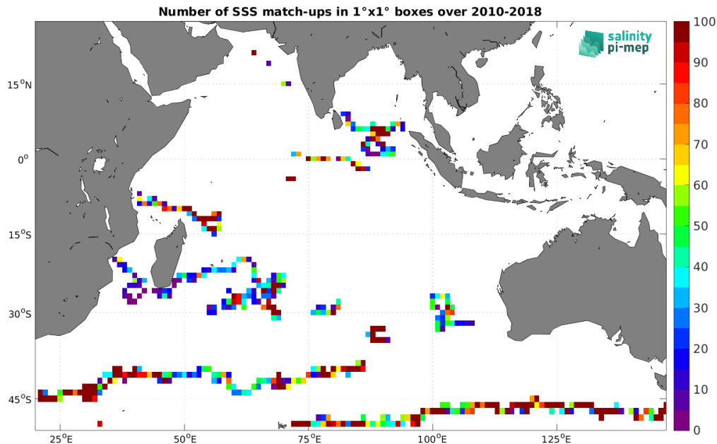
Figure 4: Number of SSS match-ups between Surface drifters SSS and the CCI SSS L4 Merged-OI v4.41 - 7-day running (ESA) SSS product for the Indian Ocean Pi-MEP region over 1^\circ \times 1^\circ boxes and for the full satellite product period.
