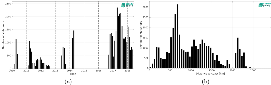
Figure 2: Number of match-ups between Surface drifters and CCI SSS L4 Merged-OI v4.41 - 7-day running (ESA) SSS as a function of time (a) and as function of the distance to coast (b) over the Indian Ocean Pi-MEP region and for the full satellite product period.
