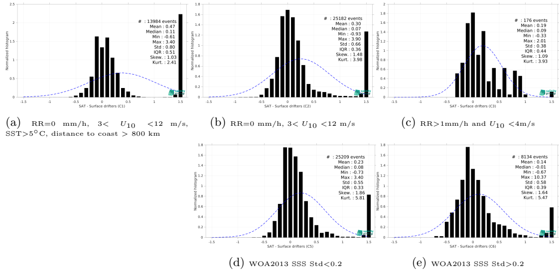
Figure 14: Normalized histogram of \Delta SSS (CCI SSS L4 Merged-OI v4.41 - 7-day running (ESA) - Surface drifters) for 5 different subdatasets corresponding to: RR=0 mm/h, 3 < U_{10} < 12 m/s, SST>5°C, distance to coast > 800 km (a), RR=0 mm/h, 3 < U_{10} < 12 m/s (b), RR>1mm/h and U_{10} < 4 m/s (c), WOA2013 SSS Std<0.2 (d), WOA2013 SSS Std>0.2 (e).
