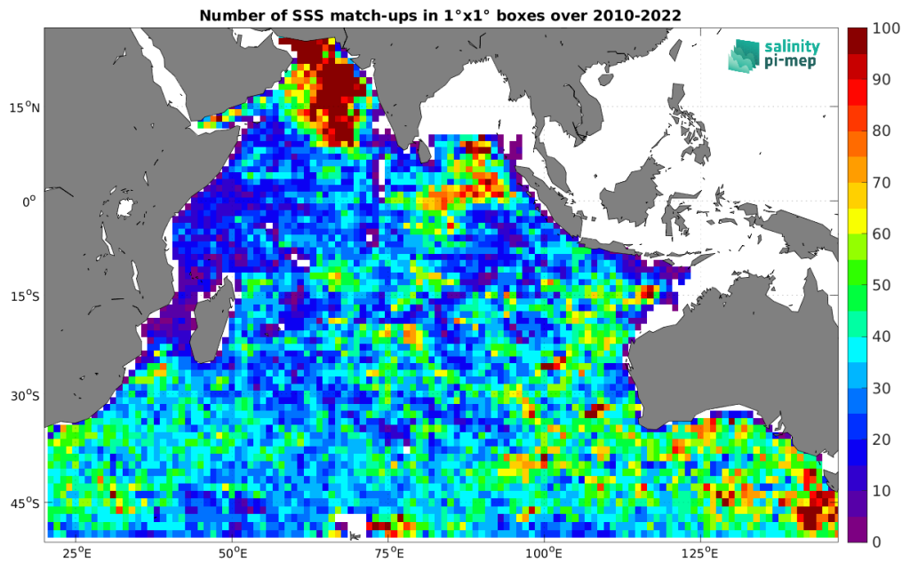
Figure 5: Number of SSS match-ups between Argo SSS and the CCI SSS L4 Merged-OI v4.41 - 7-day running (ESA) SSS product for the Indian Ocean Pi-MEP region over 1^\circ \times 1^\circ boxes and for the full satellite product period.
