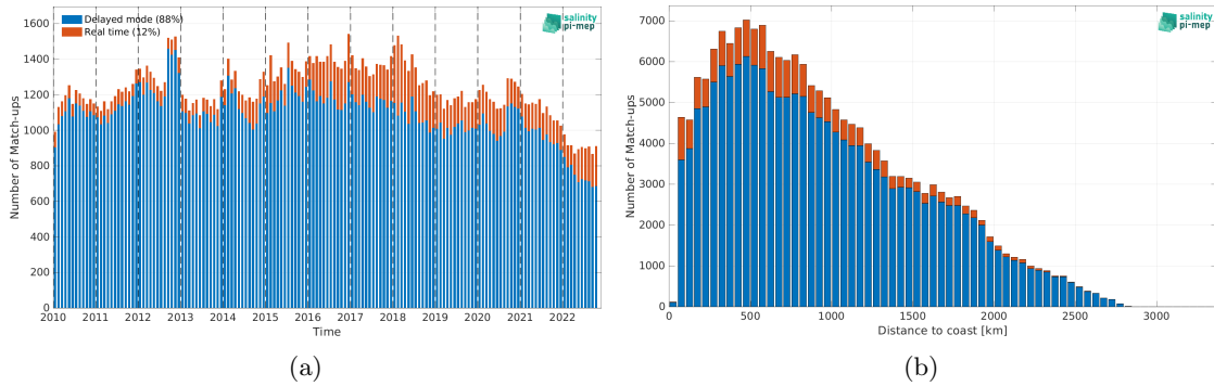
Figure 2: Number of match-ups between Argo and CCI SSS L4 Merged-OI v4.41 - 7-day running (ESA) SSS as a function of time (a) and as function of the distance to coast (b) over the Indian Ocean Pi-MEP region and for the full satellite product period.
