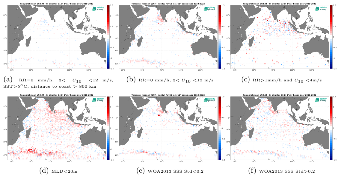
Figure 14: Temporal mean gridded over spatial boxes of size 1^\circ \times 1^\circ of \Delta SSS (CCI SSS L4 Merged-OI v4.41 - 7-day running (ESA) - Argo) for 6 different subdatasets corresponding to:RR=0 mm/h, 3 < U_{10} < 12 m/s, SST >5^\circ C, distance to coast > 800 km (a), RR=0 mm/h, 3 < U_{10} < 12 m/s (b), RR >1 mm/h and U_{10} < 4 m/s (c),MLD <20 m (d),WOA2013 SSS Std <0.2 (e),WOA2013 SSS Std >0.2 (f).
