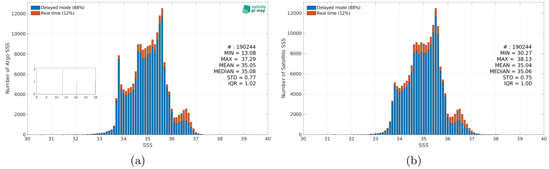
Figure 3: Histograms of SSS from Argo (a) and CCI SSS L4 Merged-OI v4.41 - 7-day running (ESA) (b) considering all match-up pairs per bins of 0.1 over the Indian Ocean Pi-MEP region and for the full satellite product period.
